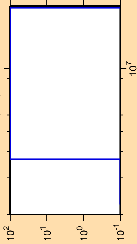
\Delta\sigma/\sigma vs. E for ^{177}\text{Re}(n,d)
