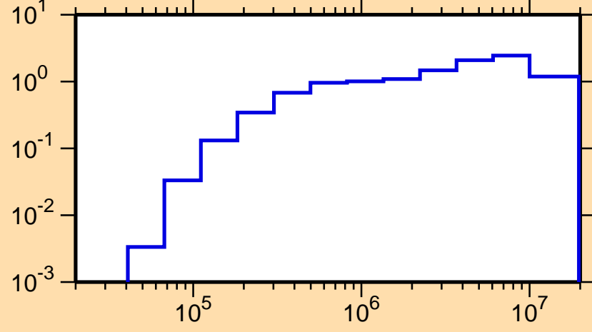
\sigma vs. E for ^{177}\text{Re}(n,\text{inel.})
