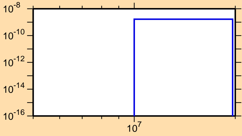
\sigma vs. E for ^{177}\text{Re}(\text{mt } 45)
