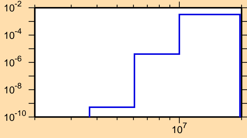
\sigma vs. E for ^{177}\text{Re}(n,d)
