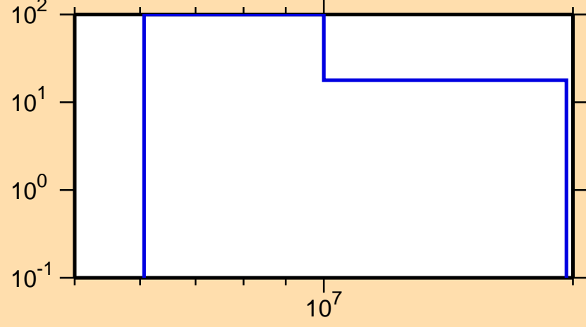
\Delta\sigma/\sigma vs. E for ^{177}\text{Re}(n,2n)
