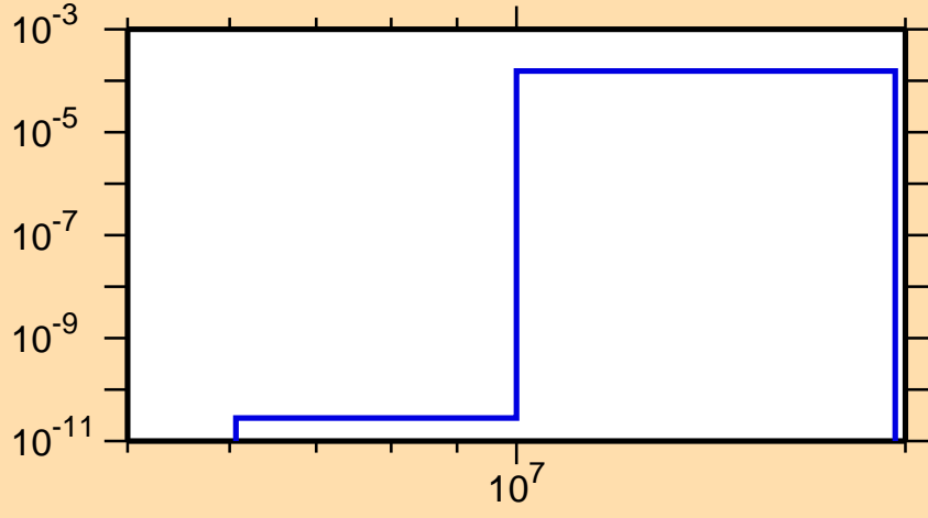
\sigma vs. E for ^{177}\text{Re}(n,t)
