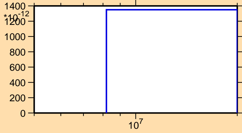
\sigma vs. E for ^{177}\text{Re}(\text{mt } 45)
