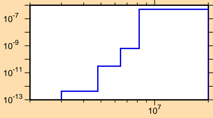
\sigma vs. E for ^{177}\text{Re}(n,p\alpha)
