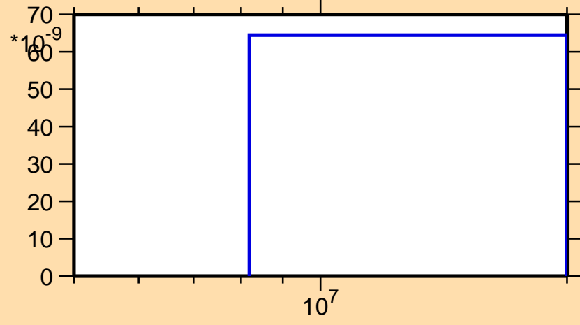
\sigma vs. E for ^{177}\text{Re}(n,2n\alpha)
