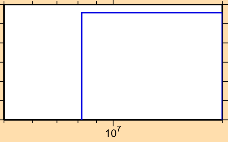
\sigma vs. E for ^{177}\text{Re}(n,3n)
