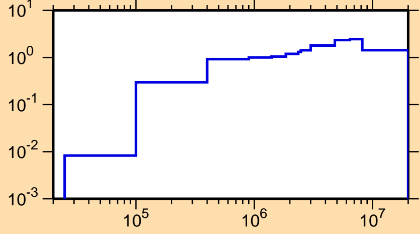
\sigma vs. E for ^{177}\text{Re}(n,\text{inel.})
