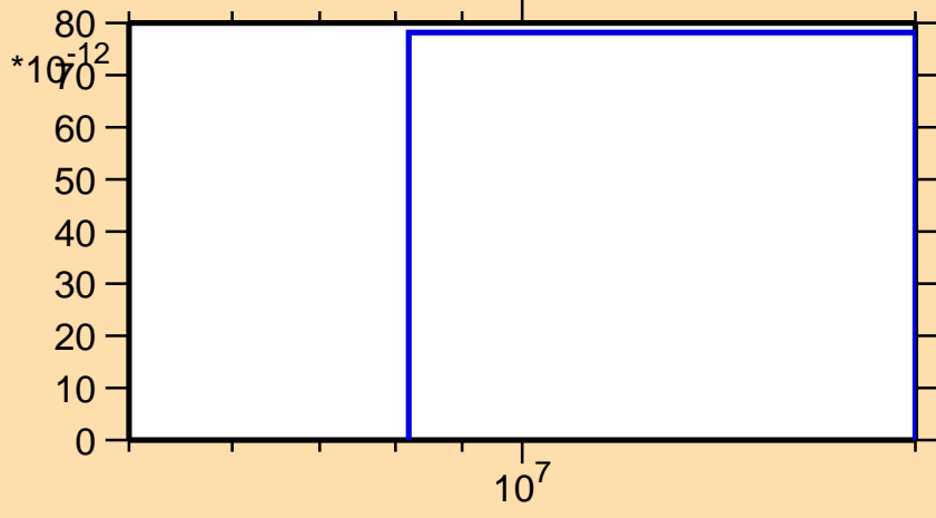
\sigma vs. E for ^{177}\text{Re}(\text{mt117})
