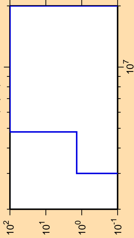
\Delta\sigma/\sigma vs. E for ^{177}\text{Re}(n,p\alpha)
