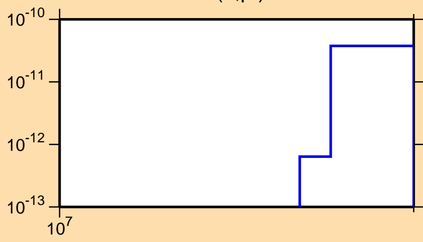
\sigma vs. E for ^{178}\text{Re}(n,\text{pt})
