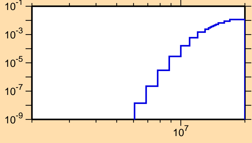
\sigma vs. E for ^{178}\text{Re}(n,d)
