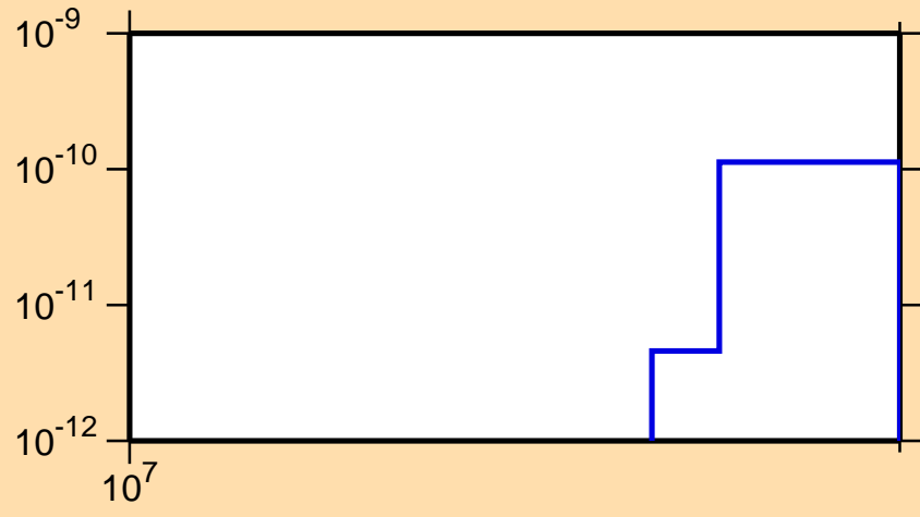
\sigma vs. E for ^{178}\text{Re}(n,pd)
