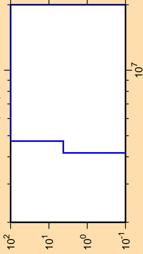
\Delta\sigma/\sigma vs. E for ^{178}\text{Re}(n,d)
