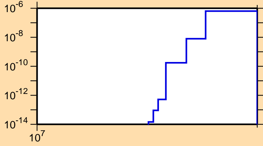
\sigma vs. E for ^{178}\text{Re}(n,nt)
