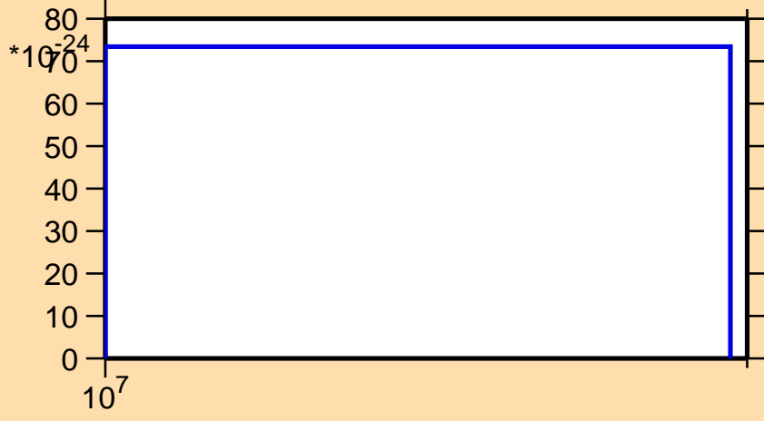
\sigma vs. E for ^{178}\text{Re}(\text{mt } 42)
