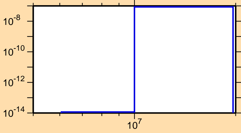
\sigma vs. E for ^{178}\text{Re}(n,\text{He3})
