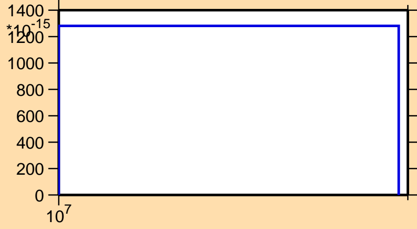
\sigma vs. E for ^{178}\text{Re}(n,\text{pd})
