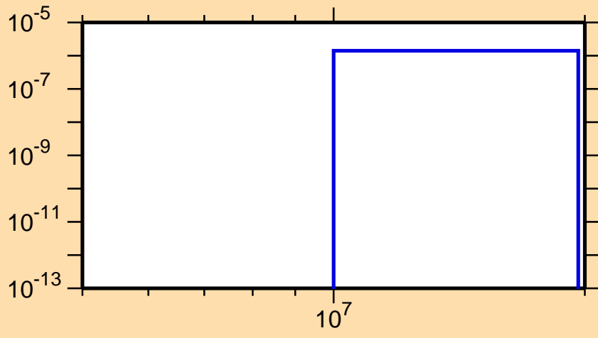
\sigma vs. E for ^{178}\text{Re}(n,2n\alpha)
