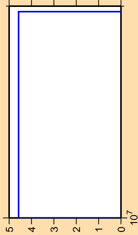
\Delta\sigma/\sigma vs. E for ^{178}\text{Re}(\text{mt } 34)
