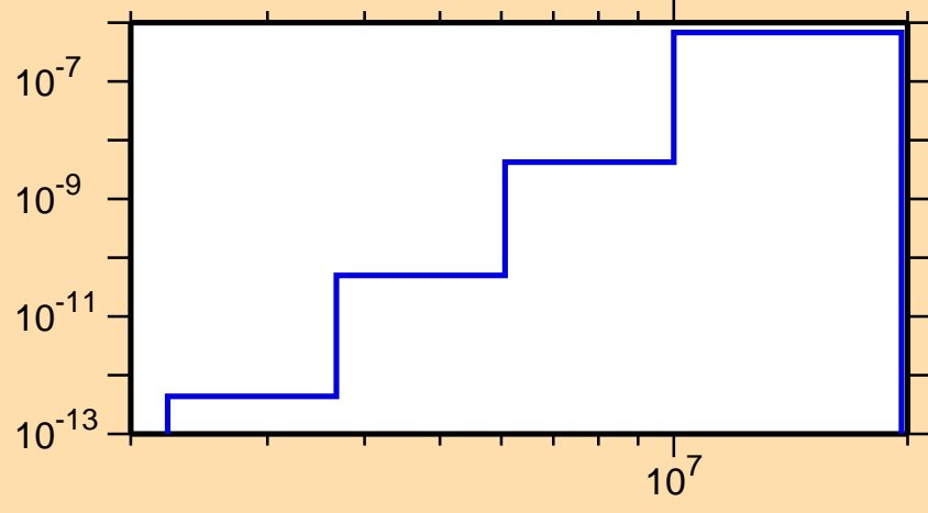
\sigma vs. E for ^{178}\text{Re}(n,p\alpha)
