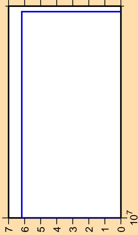
\Delta\sigma/\sigma vs. E for ^{178}\text{Re}(n,\text{pd})
