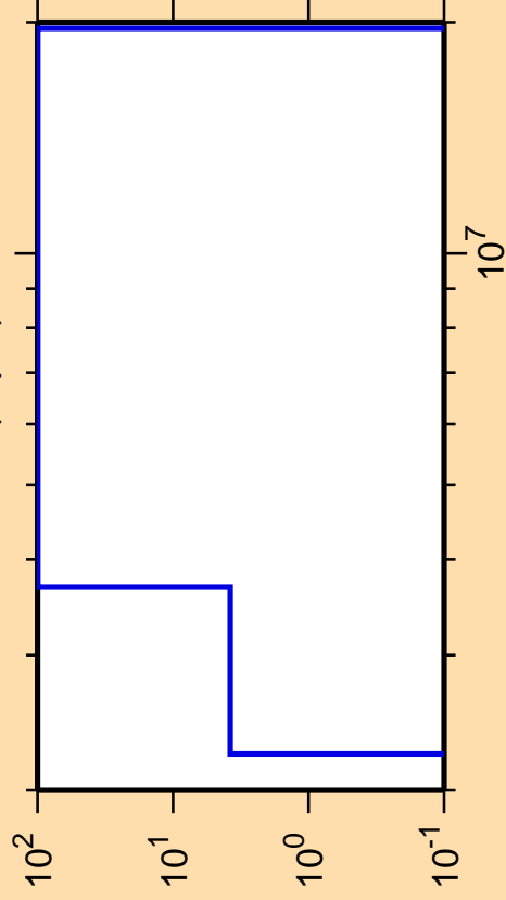
\Delta\sigma/\sigma vs. E for ^{178}\text{Re}(n,p\alpha)
