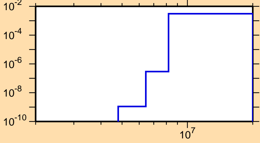
\sigma vs. E for ^{178}\text{Re}(n,d)
