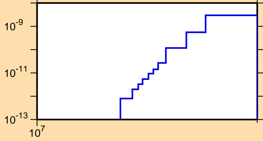
\sigma vs. E for ^{179}\text{Re}(\text{mt } 45)
