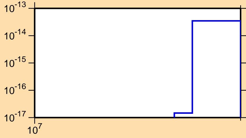
\sigma vs. E for ^{179}\text{Re}(n,\text{pt})
