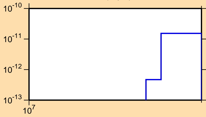
\sigma vs. E for ^{179}\text{Re}(n,\text{pd})
