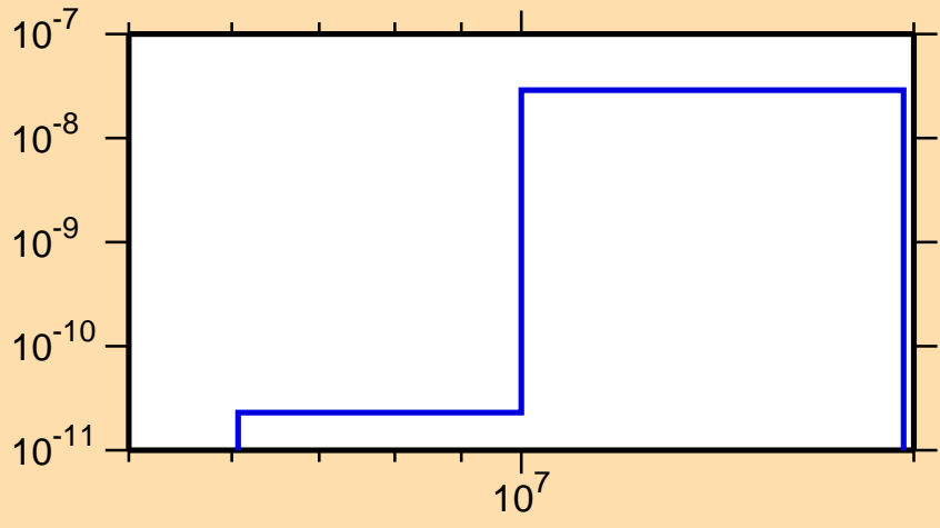
\sigma vs. E for ^{179}\text{Re}(n,p\alpha)
