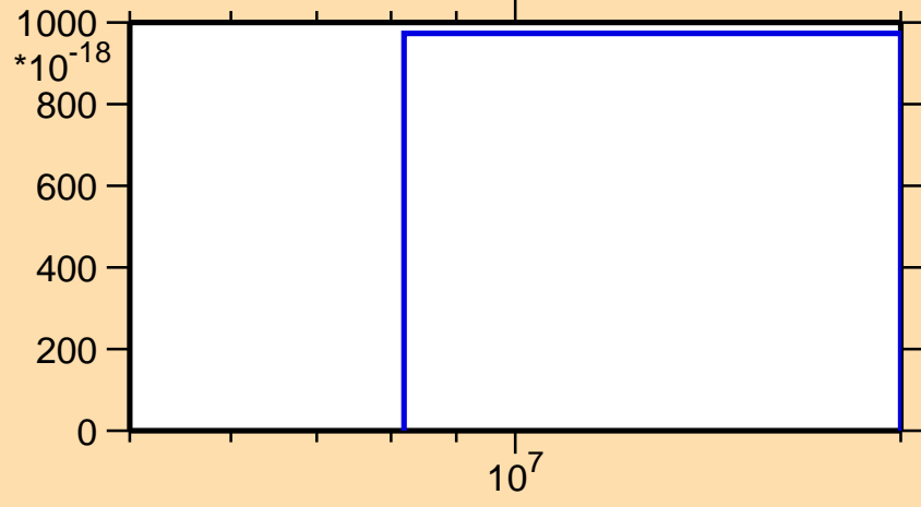
\sigma vs. E for ^{179}\text{Re}(n,3n\alpha)
