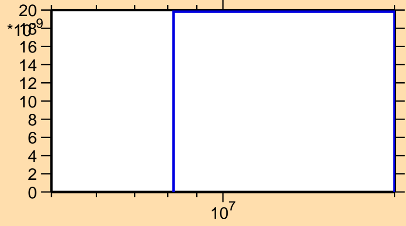
\sigma vs. E for ^{179}\text{Re}(n,2n\alpha)
