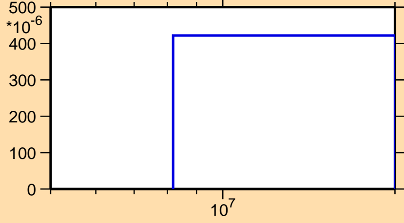
\sigma vs. E for ^{179}\text{Re}(n,3n)
