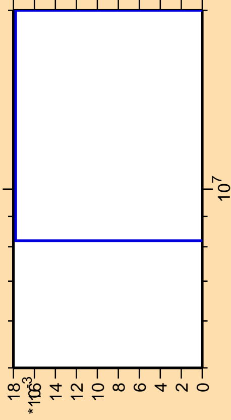
\Delta\sigma/\sigma vs. E for ^{179}\text{Re}(\text{mt } 34)
