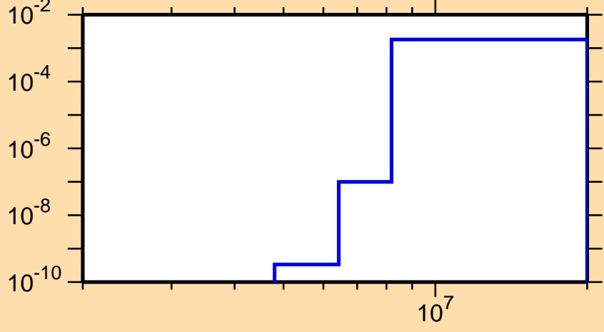
\sigma vs. E for ^{179}\text{Re}(n,d)
