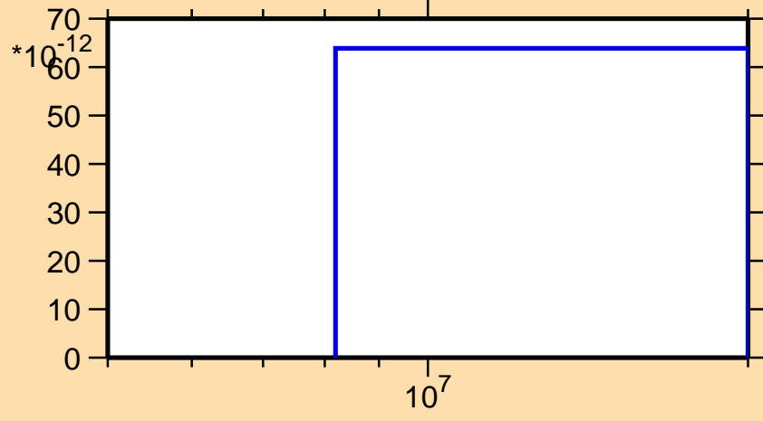
\sigma vs. E for ^{179}\text{Re}(\text{mt } 45)
