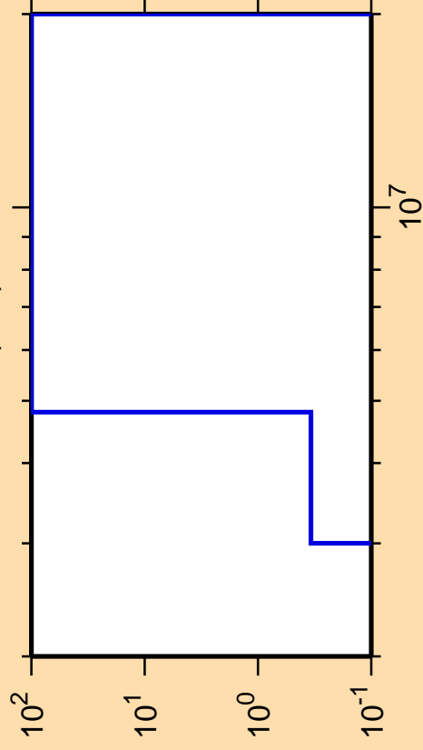
\Delta\sigma/\sigma vs. E for ^{179}\text{Re}(n,d)
