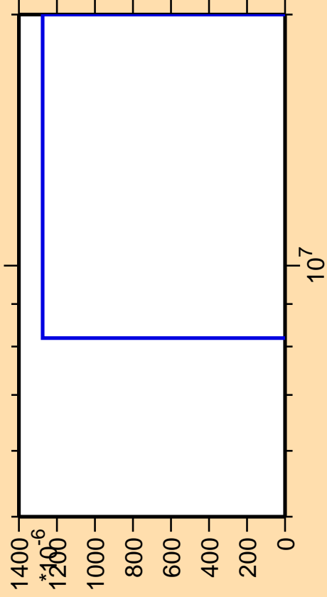
\Delta\sigma/\sigma vs. E for ^{179}\text{Re}(n,3n\alpha)
