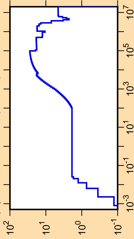
\Delta\mu/\mu vs. E for ^{180}\text{Re}(\text{mt251})
