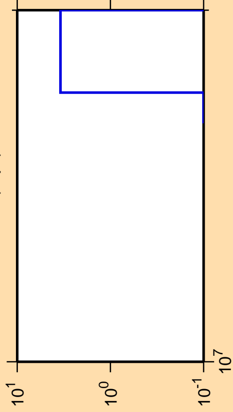
\Delta\sigma/\sigma vs. E for ^{180}\text{Re}(n,\text{pt})
