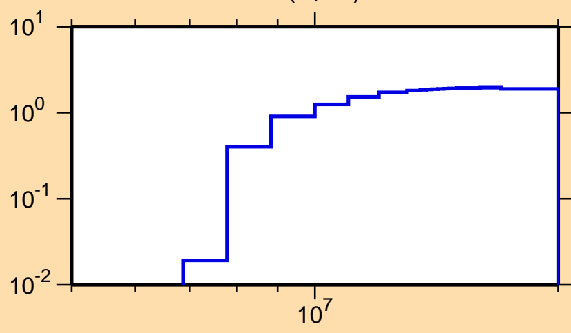
\sigma vs. E for ^{180}\text{Re}(n,2n)
