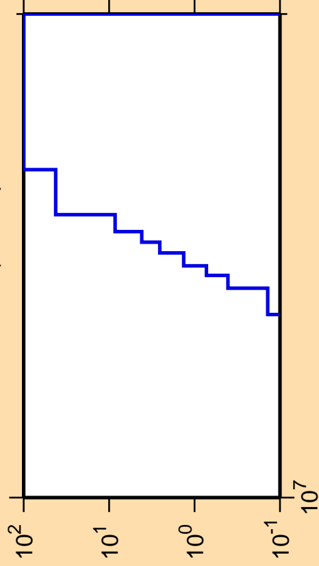
\Delta\sigma/\sigma vs. E for ^{180}\text{Re}(mt\ 45)
