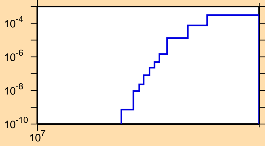
\sigma vs. E for ^{180}\text{Re}(n,2np)
