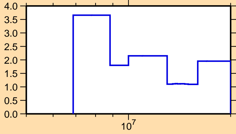
\Delta\sigma/\sigma vs. E for ^{180}\text{Re}(n,\text{tot.})
