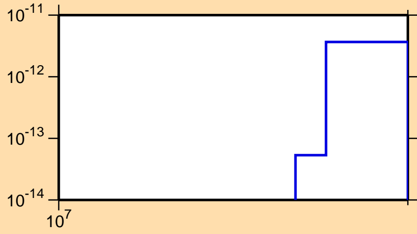
\sigma vs. E for ^{180}\text{Re}(n,\text{pd})
