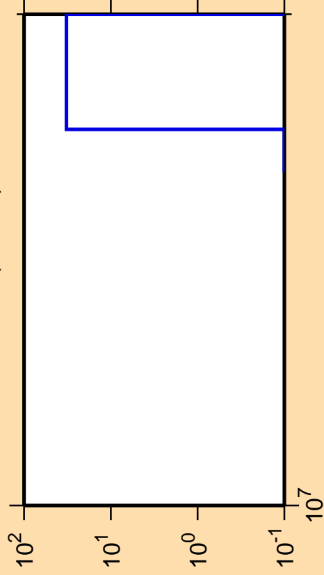
\Delta\sigma/\sigma vs. E for ^{180}\text{Re}(\text{mt } 34)
