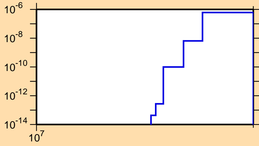
\sigma vs. E for ^{180}\text{Re}(n,nt)
