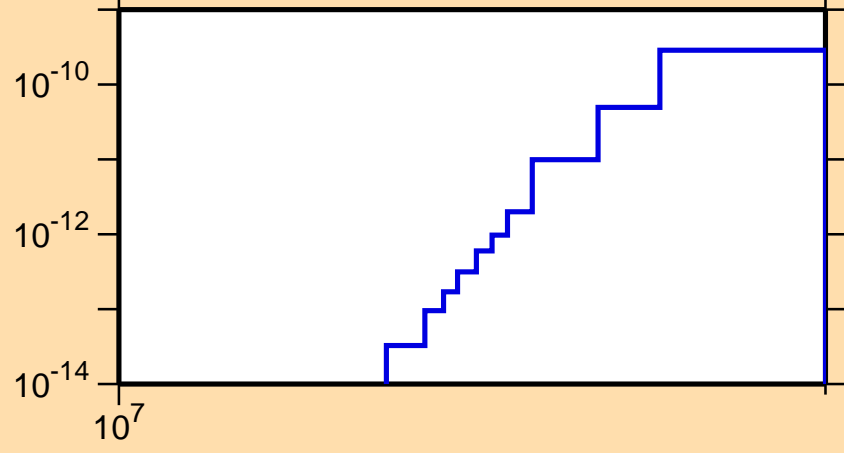
\sigma vs. E for ^{180}\text{Re}(mt\ 45)
