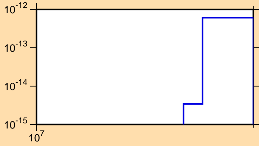
\sigma vs. E for ^{180}\text{Re}(n,\text{pt})
