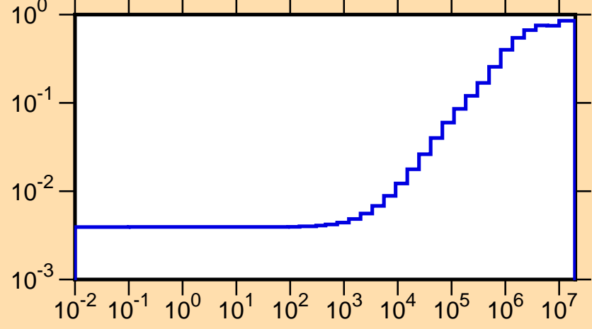
\mu vs. E for ^{180}\text{Re}(\text{mt251})
