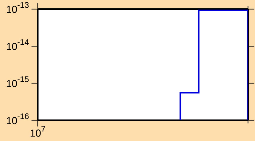
\sigma vs. E for ^{181}\text{Re}(n,\text{pd})
