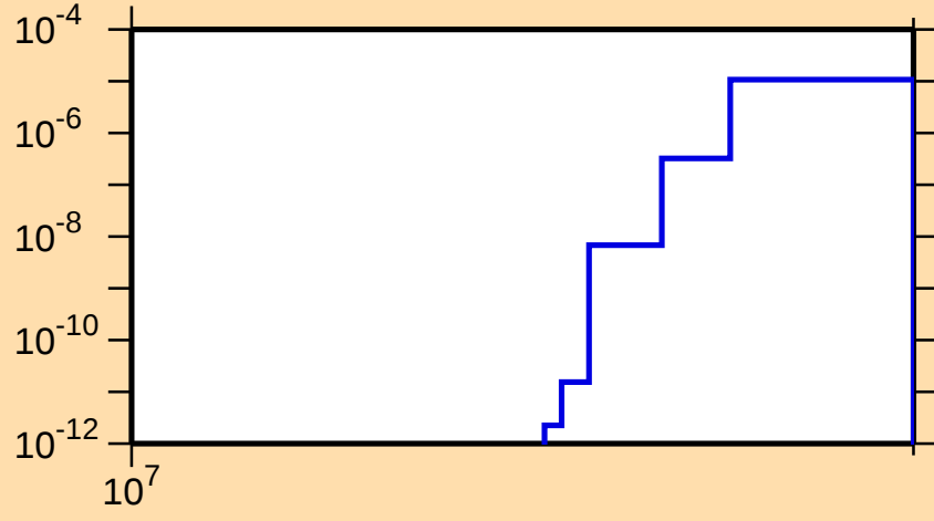
\sigma vs. E for ^{181}\text{Re}(n,2np)
