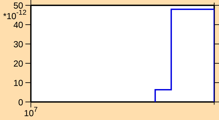
\sigma vs. E for ^{181}\text{Re}(\text{mt 45})
