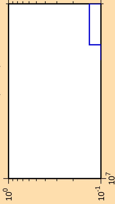
\Delta\sigma/\sigma vs. E for ^{181}\text{Re}(n,3n\alpha)
