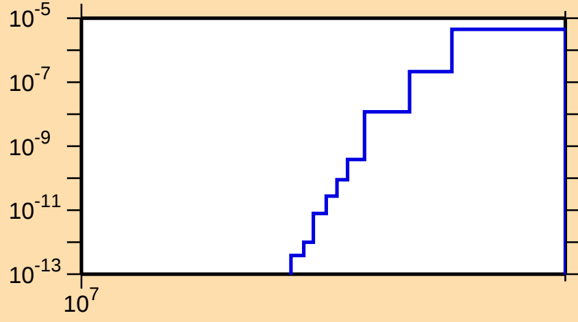
\sigma vs. E for ^{181}\text{Re}(n,\text{nd})
