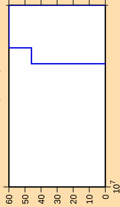
\Delta\sigma/\sigma vs. E for ^{181}\text{Re}(\text{mt 45})
