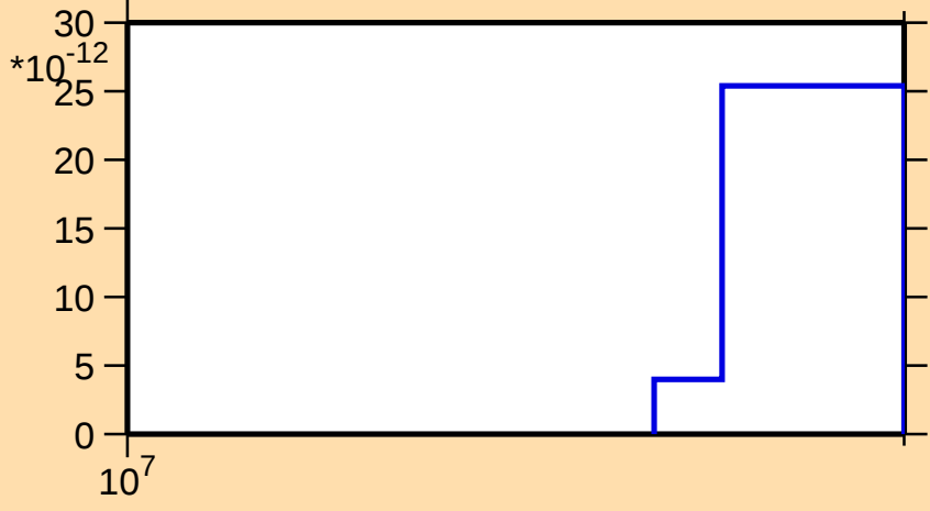
\sigma vs. E for ^{181}\text{Re}(\text{mt117})
