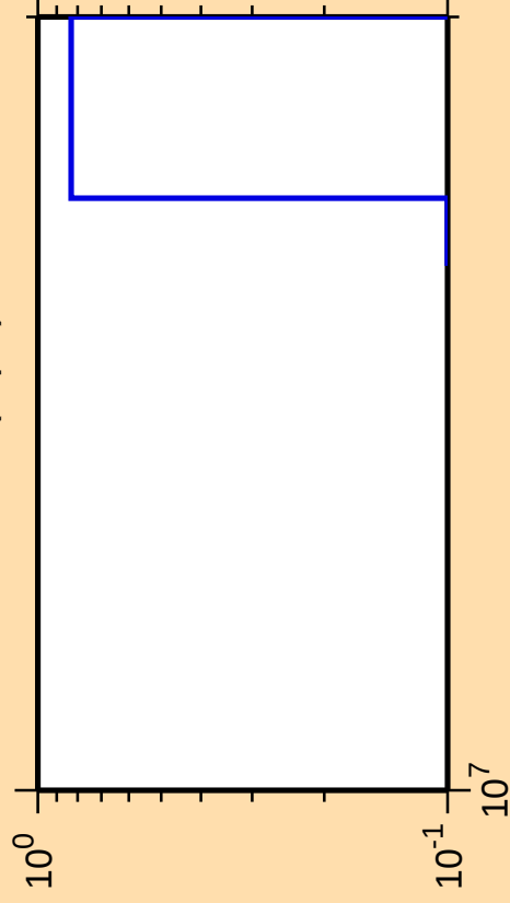
\Delta\sigma/\sigma vs. E for ^{181}\text{Re}(n,\text{pd})
