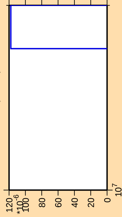
\Delta\sigma/\sigma vs. E for ^{181}\text{Re}(\text{mt } 42)
