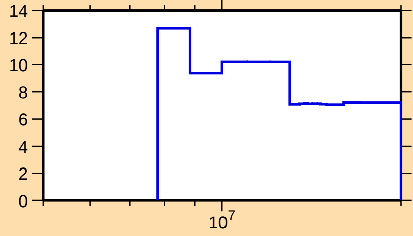
\Delta\sigma/\sigma vs. E for ^{181}\text{Re}(n,\text{el.})
