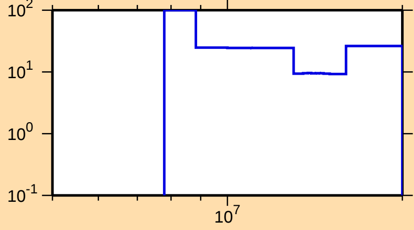
\Delta\sigma/\sigma vs. E for ^{181}\text{Re}(n,2n)
