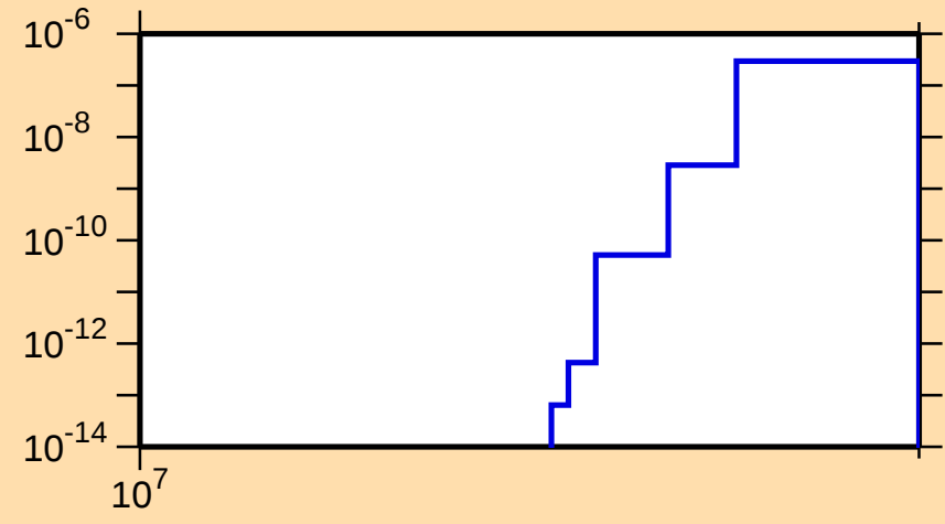
\sigma vs. E for ^{181}\text{Re}(n,nt)
