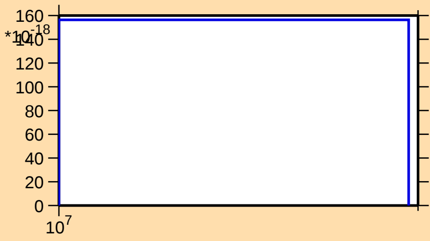
\sigma vs. E for ^{181}\text{Re}(n,3n\alpha)
