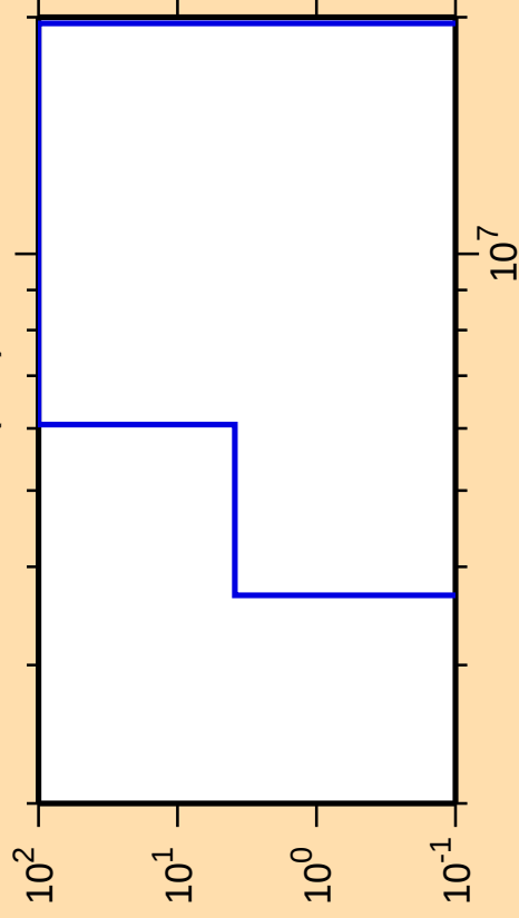
\Delta\sigma/\sigma vs. E for ^{181}\text{Re}(n,d)
