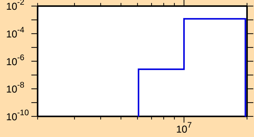
\sigma vs. E for ^{181}\text{Re}(n,d)
