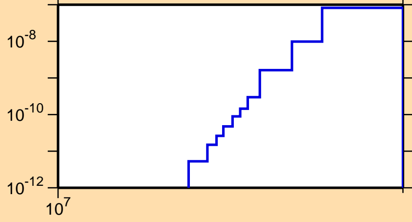
\sigma vs. E for ^{182}\text{Re}(n,\text{He}3)
