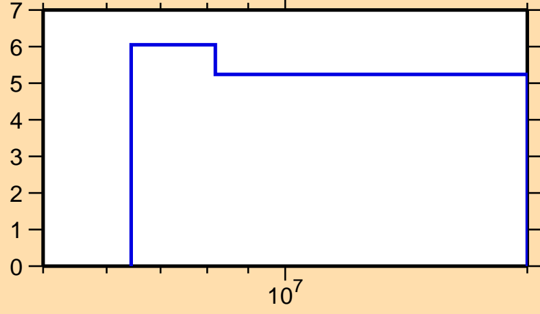
\Delta\sigma/\sigma vs. E for ^{182}\text{Re}(n,\text{tot.})
