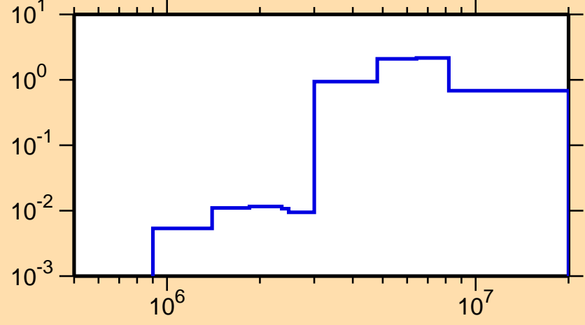
\sigma vs. E for ^{182}\text{Re}(n,n\text{cont.})
