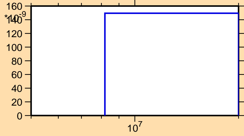
\sigma vs. E for ^{182}\text{Re}(n,2n\alpha)
