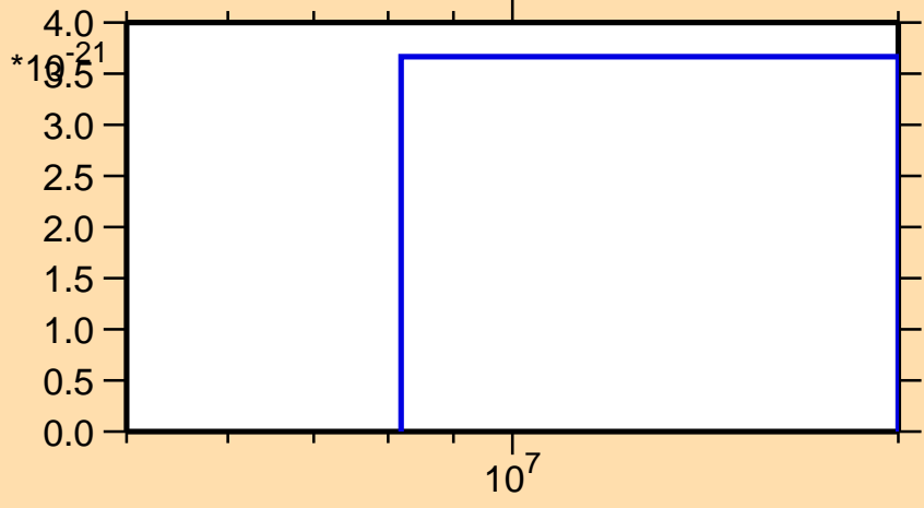
\sigma vs. E for ^{182}\text{Re}(\text{mt } 42)
