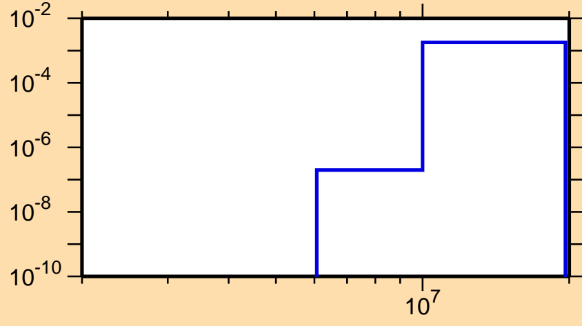
\sigma vs. E for ^{182}\text{Re}(n,d)
