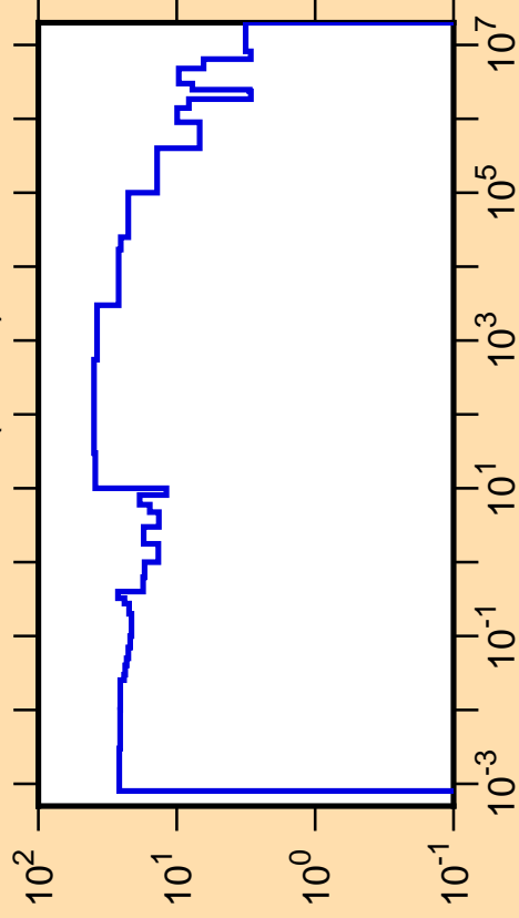
\Delta\sigma/\sigma vs. E for ^{182}\text{Re}(n,\text{tot.})
