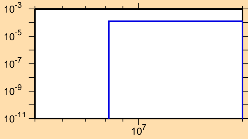
\sigma vs. E for ^{182}\text{Re}(n,t)
