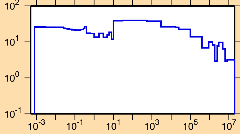
\Delta\sigma/\sigma vs. E for ^{182}\text{Re}(n,\text{tot.})
