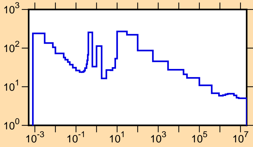
\sigma vs. E for ^{182}\text{Re}(n,\text{tot.})
