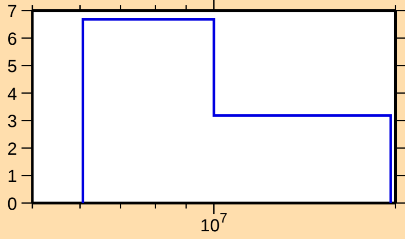
\Delta\sigma/\sigma vs. E for ^{183}\text{Re}(n,\text{tot.})
