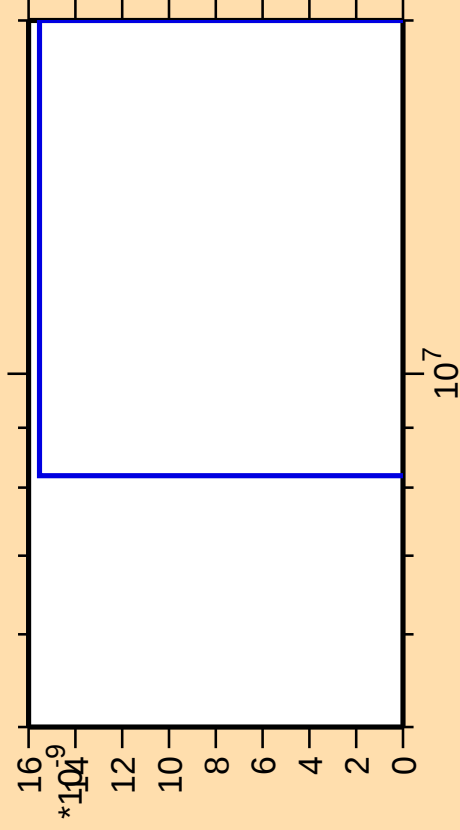
\Delta\sigma/\sigma vs. E for ^{183}\text{Re}(\text{mt } 42)
