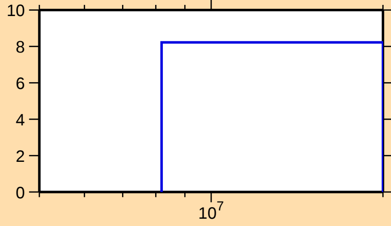
\Delta\sigma/\sigma vs. E for ^{183}\text{Re}(n,\text{nonel.})
