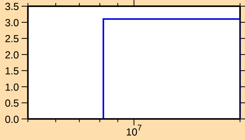
\Delta\sigma/\sigma vs. E for ^{183}\text{Re}(n,\text{tot.})
