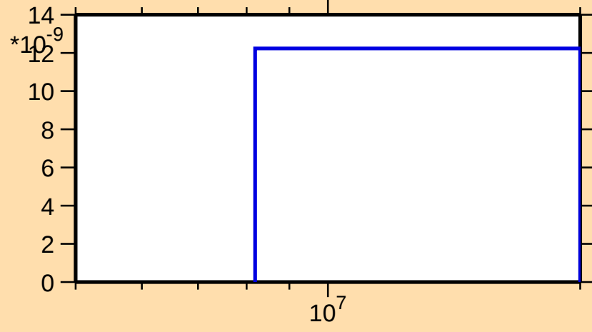
\sigma vs. E for ^{183}\text{Re}(n,2np)
