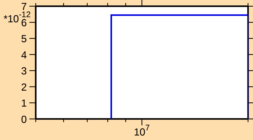
\sigma vs. E for ^{183}\text{Re}(n,p\alpha)
