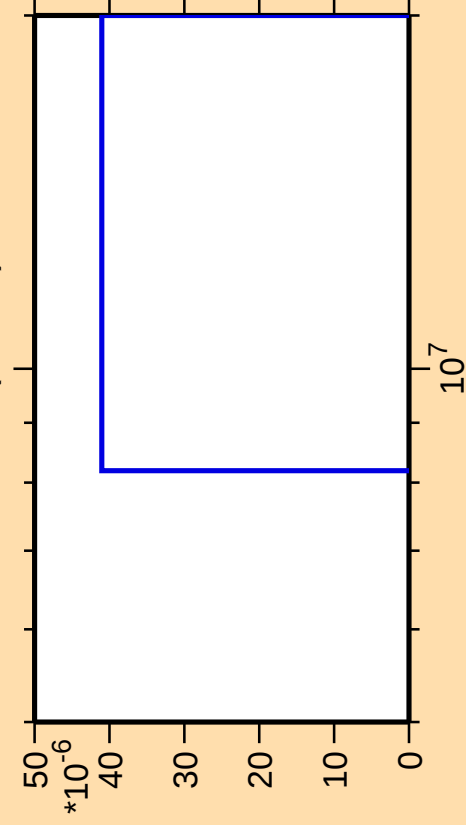
\Delta\sigma/\sigma vs. E for ^{183}\text{Re}(n,3n\alpha)
