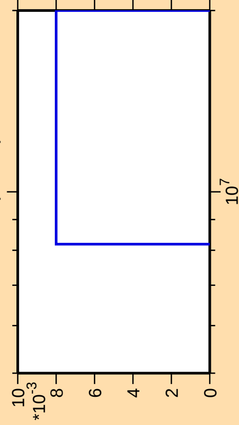
\Delta\sigma/\sigma vs. E for ^{183}\text{Re}(\text{mt } 45)
