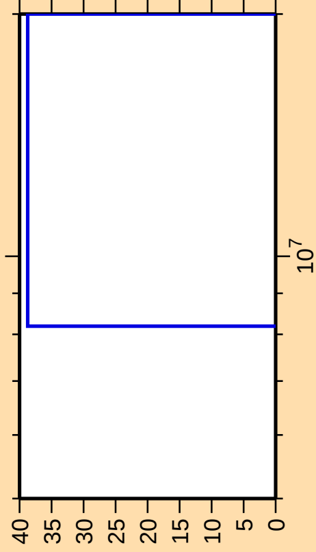
\Delta\sigma/\sigma vs. E for ^{183}\text{Re}(n,3n)
