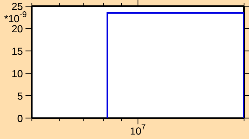
\sigma vs. E for ^{183}\text{Re}(n,\text{nd})
