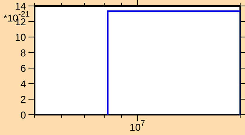
\sigma vs. E for ^{183}\text{Re}(\text{mt } 42)
