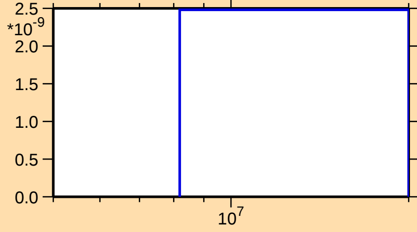
\sigma vs. E for ^{183}\text{Re}(n,nt)
