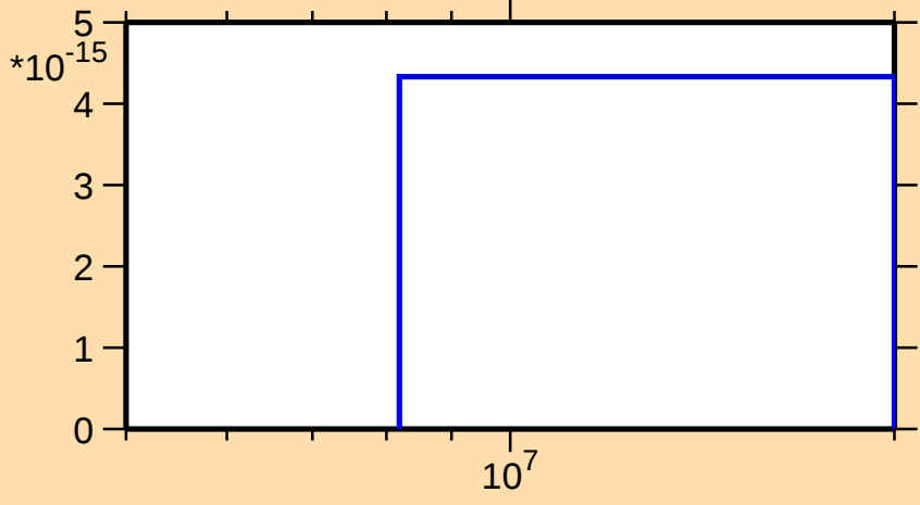
\sigma vs. E for ^{183}\text{Re}(\text{mt117})
