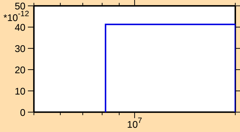
\sigma vs. E for ^{183}\text{Re}(n,\text{He3})
