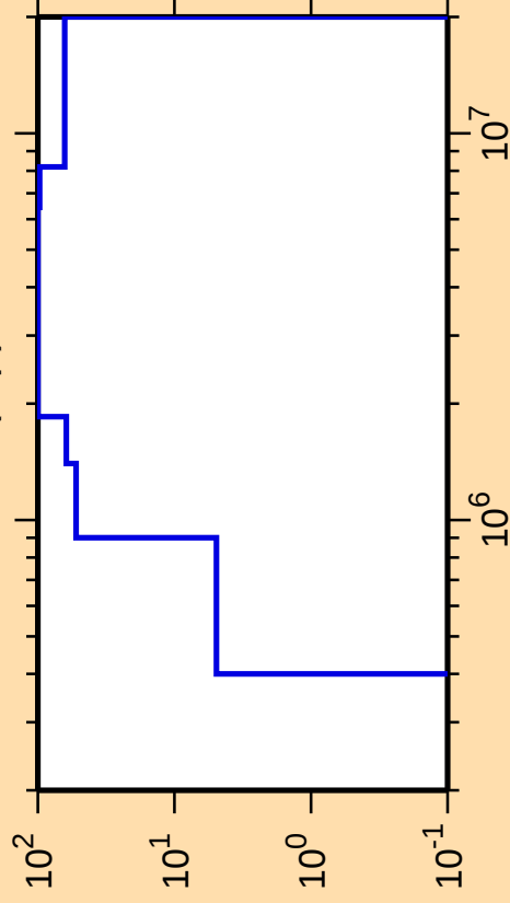
\Delta\sigma/\sigma vs. E for ^{183}\text{Re}(n,p)
