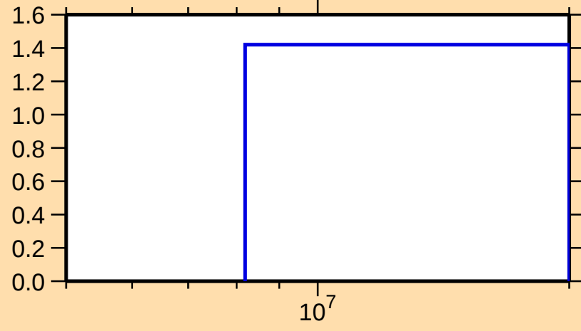
\sigma vs. E for ^{183}\text{Re}(n,2n)
