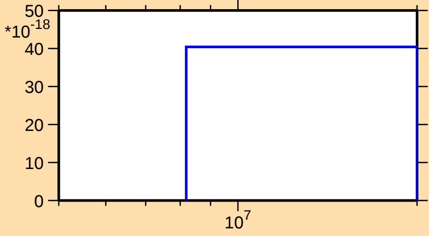
\sigma vs. E for ^{183}\text{Re}(n,3n\alpha)
