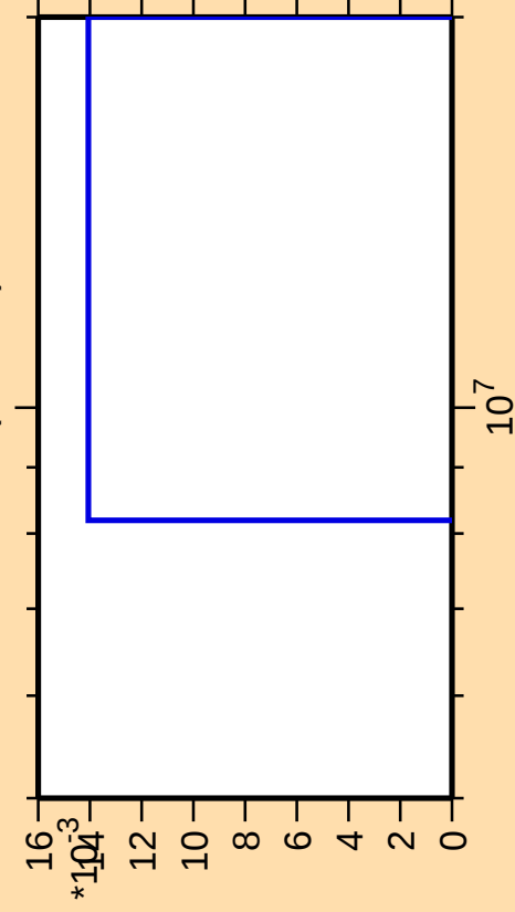
\Delta\sigma/\sigma vs. E for ^{183}\text{Re}(\text{mt117})
