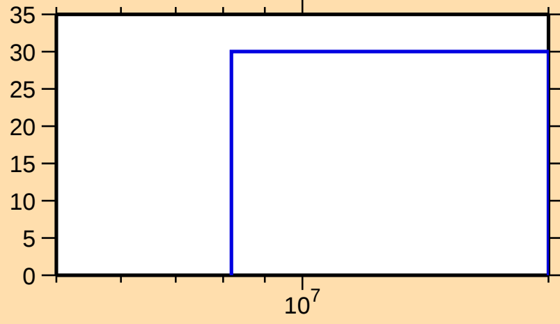
\Delta\sigma/\sigma vs. E for ^{183}\text{Re}(n,\text{inel.})
