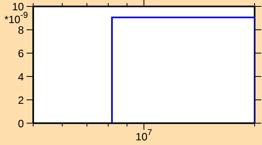
\sigma vs. E for ^{183}\text{Re}(n,2n\alpha)
