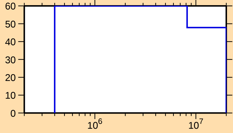
\Delta\sigma/\sigma vs. E for ^{183}\text{Re}(n,n_1)
