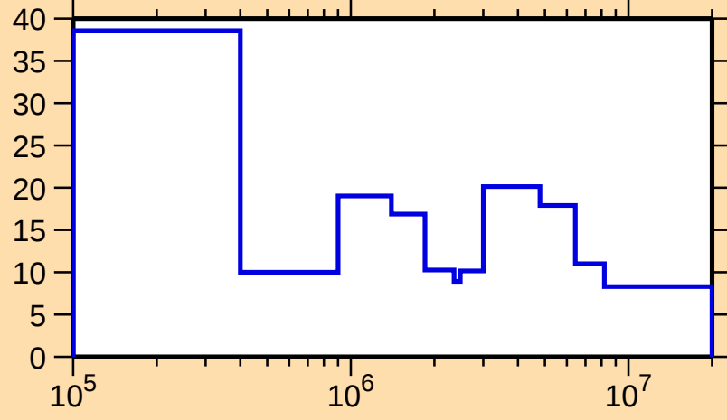
\Delta\sigma/\sigma vs. E for ^{183}\text{Re}(n,\text{el.})
