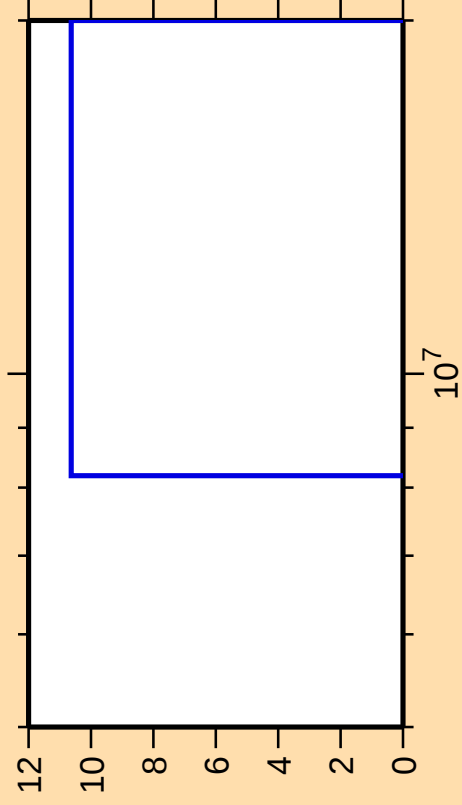
\Delta\sigma/\sigma vs. E for ^{183}\text{Re}(n,2n)
