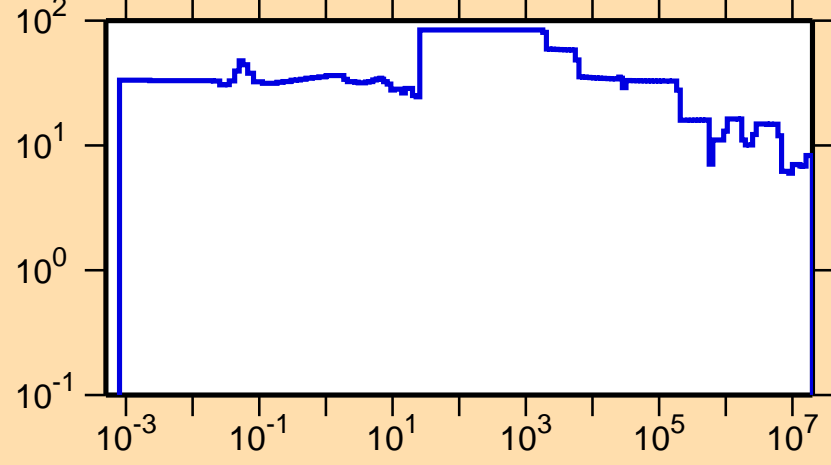
\Delta\sigma/\sigma vs. E for ^{184}\text{Re}(n,\text{el.})
