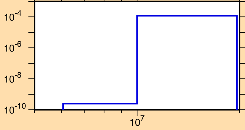
\sigma vs. E for ^{184}\text{Re}(n,t)
