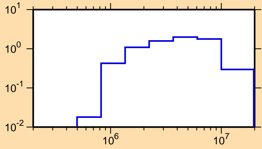
\sigma vs. E for ^{184}\text{Re}(n,n\text{cont.})
