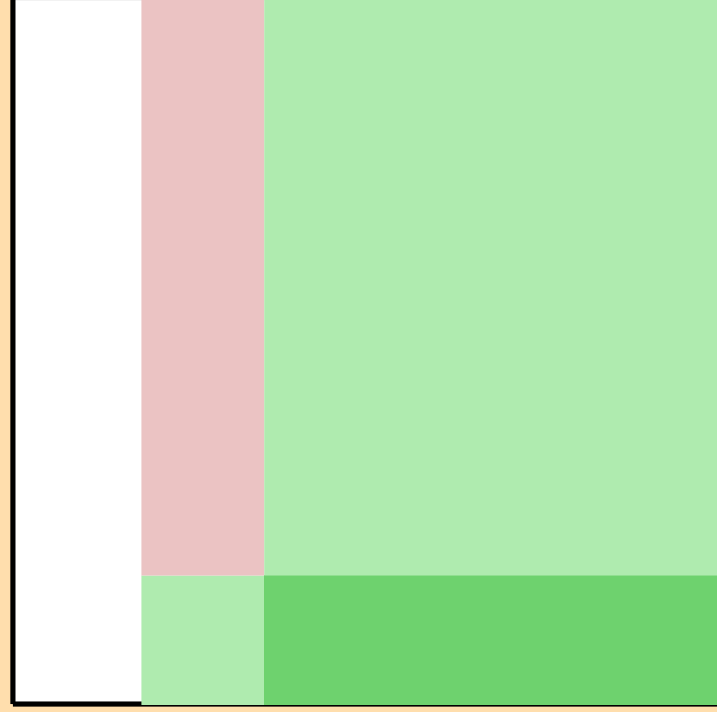
\Delta\sigma/\sigma vs. E for ^{184}\text{Re}(n,2n)
