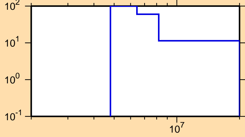
\Delta\sigma/\sigma vs. E for ^{184}\text{Re}(n,2n)
