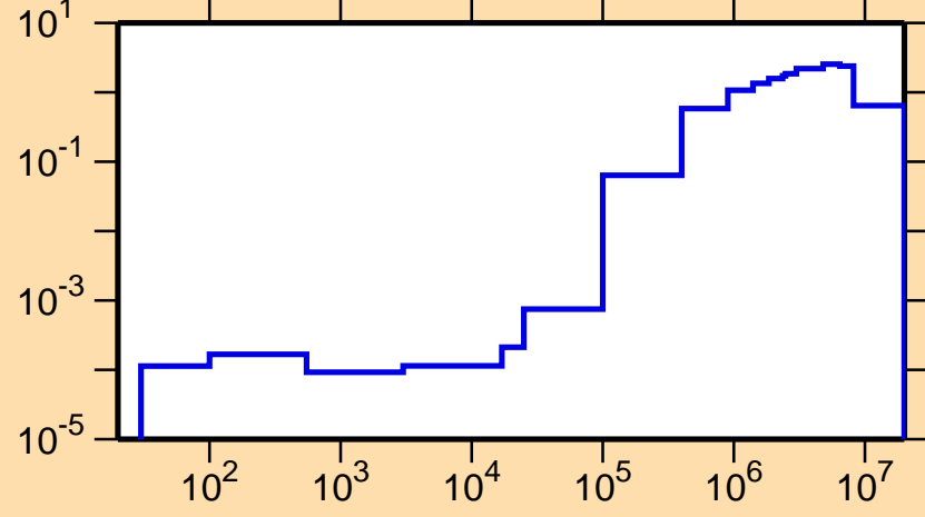
\sigma vs. E for ^{184}\text{Re}(n,\text{inel.})
