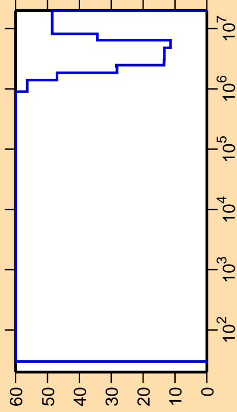
\Delta\sigma/\sigma vs. E for ^{184}\text{Re}(n,\text{inel.})
