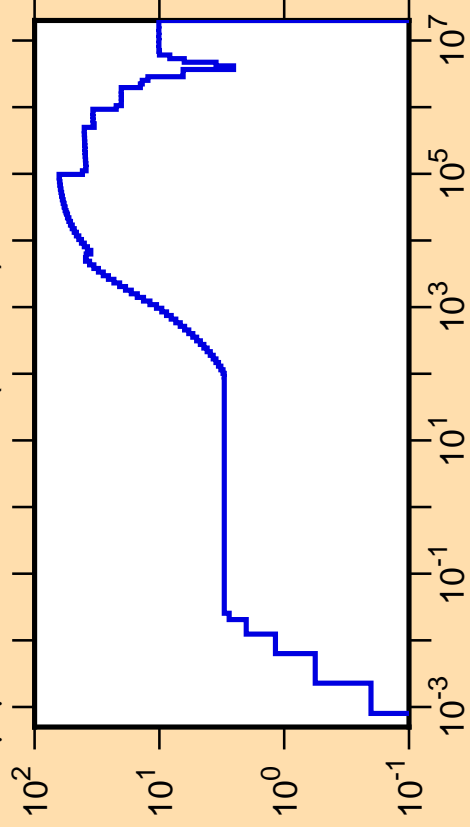
\Delta\mu/\mu vs. E for ^{186}\text{Re}(\text{mt251})
