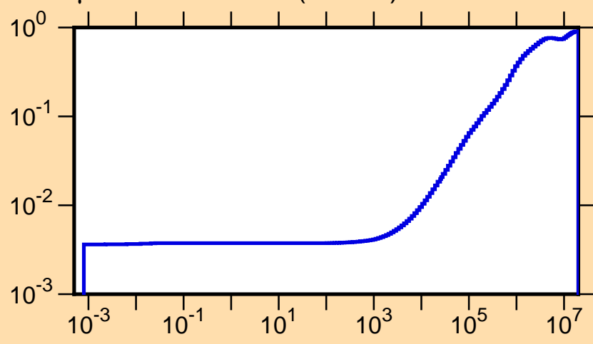
\mu vs. E for ^{186}\text{Re}(\text{mt251})
