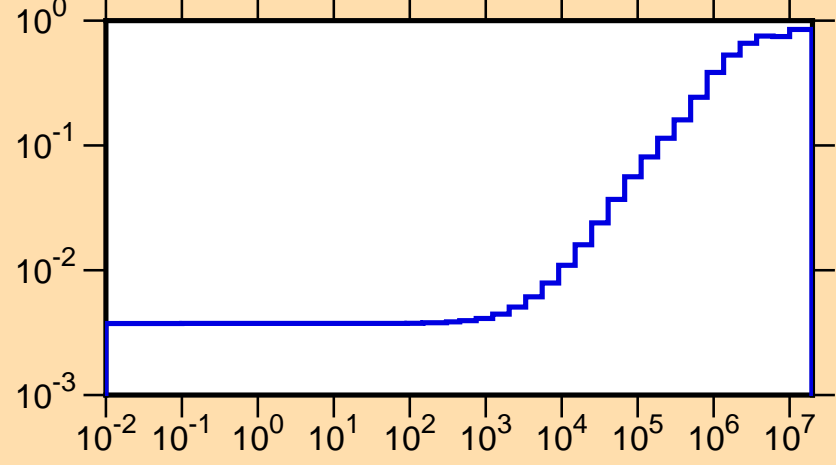
\mu vs. E for ^{186}\text{Re}(\text{mt251})
