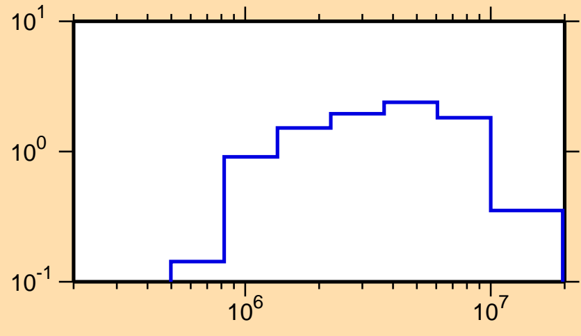
\sigma vs. E for ^{186}\text{Re}(n,n\text{cont.})
