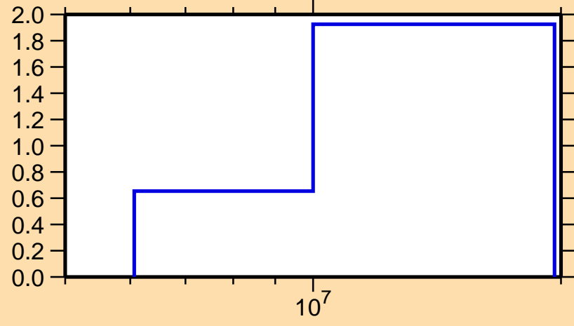
\sigma vs. E for ^{186}\text{Re}(n,2n)
