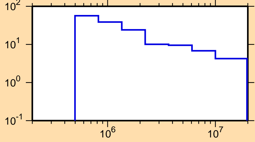
\Delta\sigma/\sigma vs. E for ^{186}\text{Re}(n,\text{nonel.})
