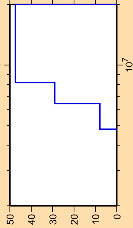
\Delta\sigma/\sigma vs. E for ^{186}\text{Re}(n,n\text{cont.})
