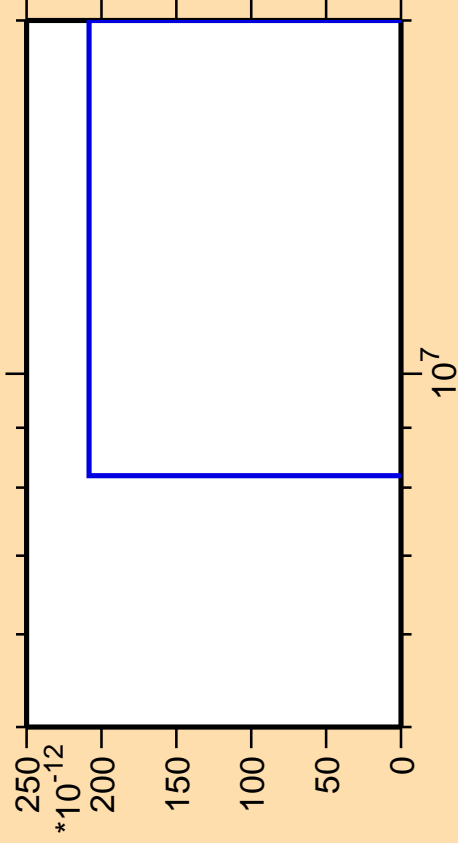
\Delta\sigma/\sigma vs. E for ^{186}\text{Re}(\text{mt } 42)
