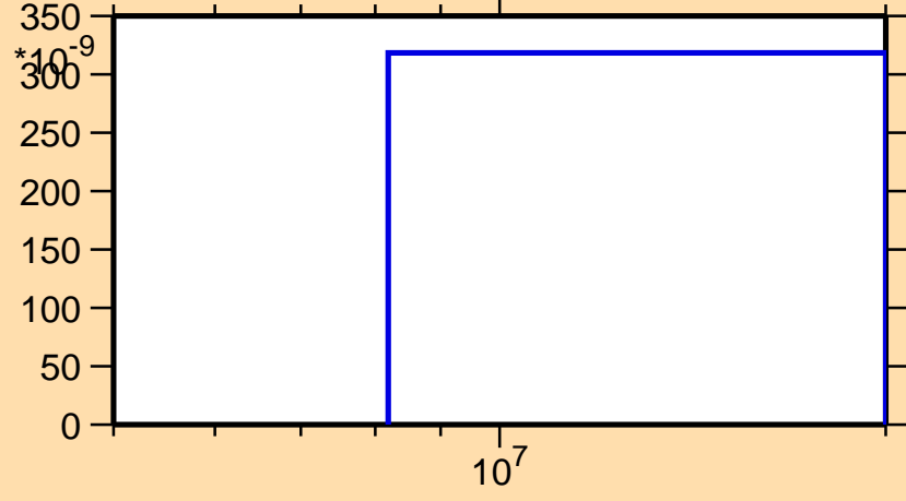
\sigma vs. E for ^{186}\text{Re}(n,\text{nd})
