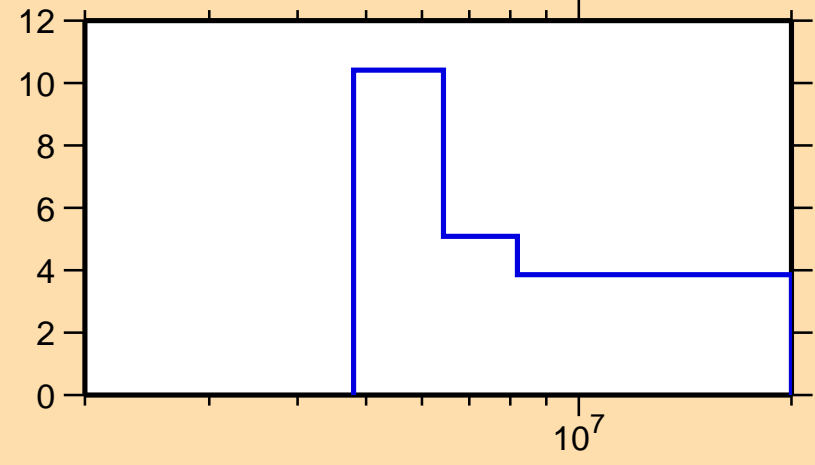
\Delta\sigma/\sigma vs. E for ^{186}\text{Re}(n,\text{tot.})
