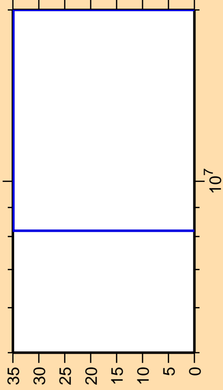
\Delta\sigma/\sigma vs. E for ^{186}\text{Re}(n,3n)
