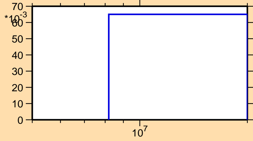
\sigma vs. E for ^{186}\text{Re}(n,3n)
