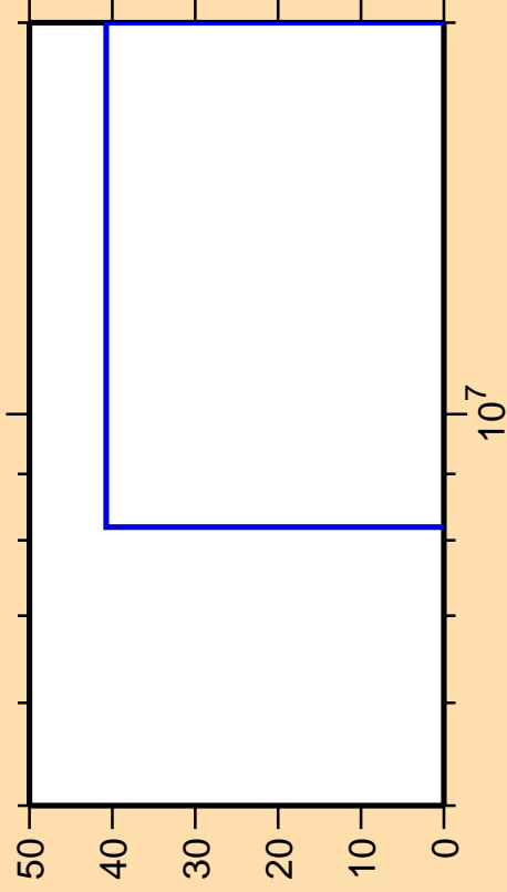
\Delta\sigma/\sigma vs. E for ^{186}\text{Re}(n,\text{He}3)
