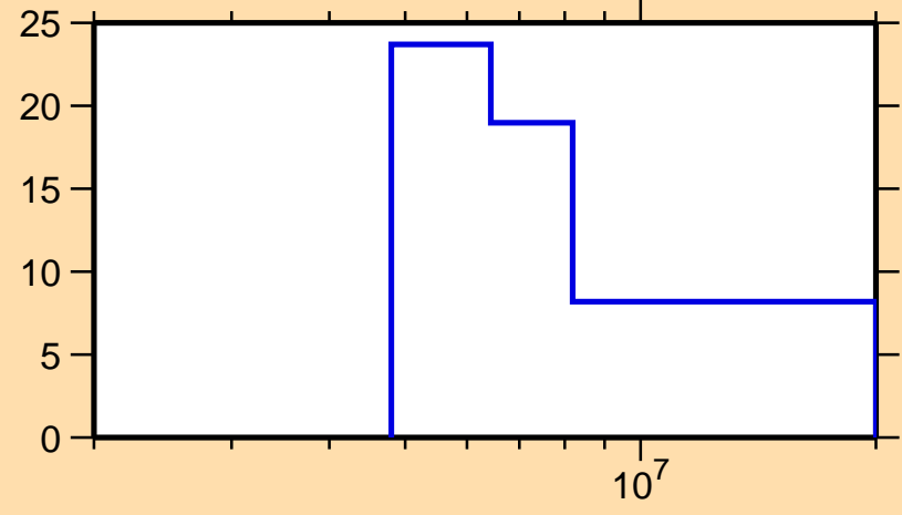
\Delta\sigma/\sigma vs. E for ^{186}\text{Re}(n,2n)
