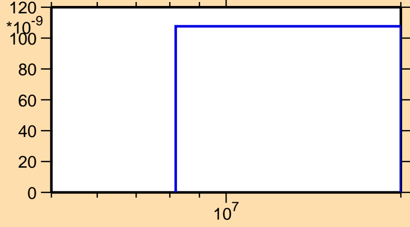
\sigma vs. E for ^{186}\text{Re}(n,2np)
