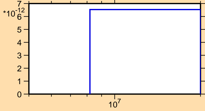
\sigma vs. E for ^{186}\text{Re}(n,\text{He}3)
