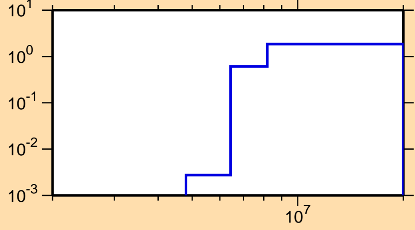
\sigma vs. E for ^{186}\text{Re}(n,2n)
