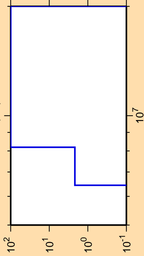
\Delta\sigma/\sigma vs. E for ^{186}\text{Re}(n,t)
