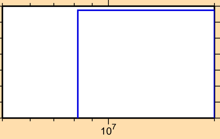
\sigma vs. E for ^{186}\text{Re}(n,2n\alpha)
