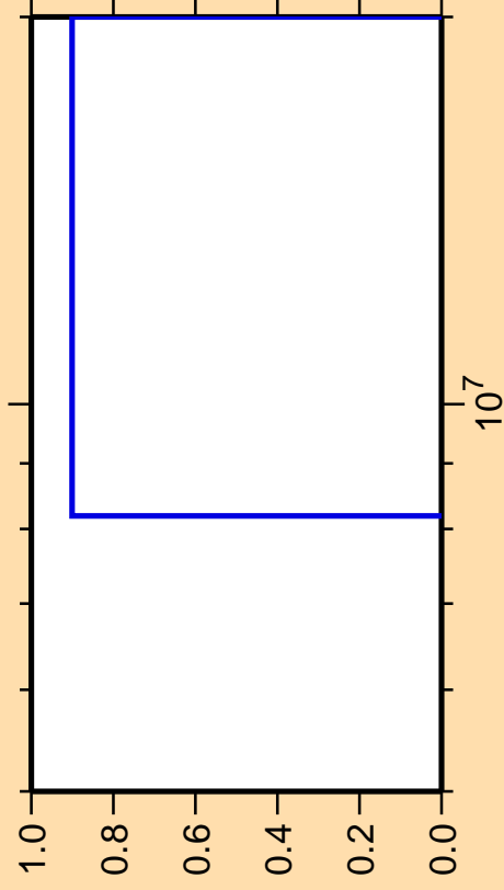
\Delta\sigma/\sigma vs. E for ^{186}\text{Re}(n,p\alpha)
