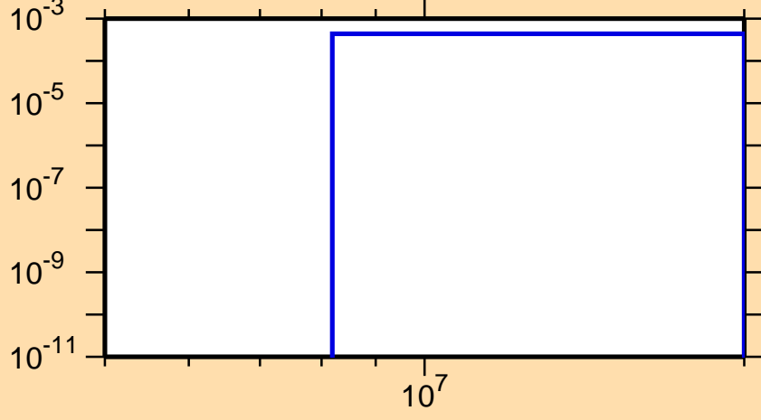
\sigma vs. E for ^{186}\text{Re}(n,np)
