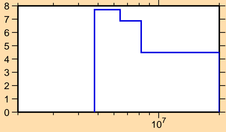
\Delta\sigma/\sigma vs. E for ^{186}\text{Re}(n,\text{nonel.})
