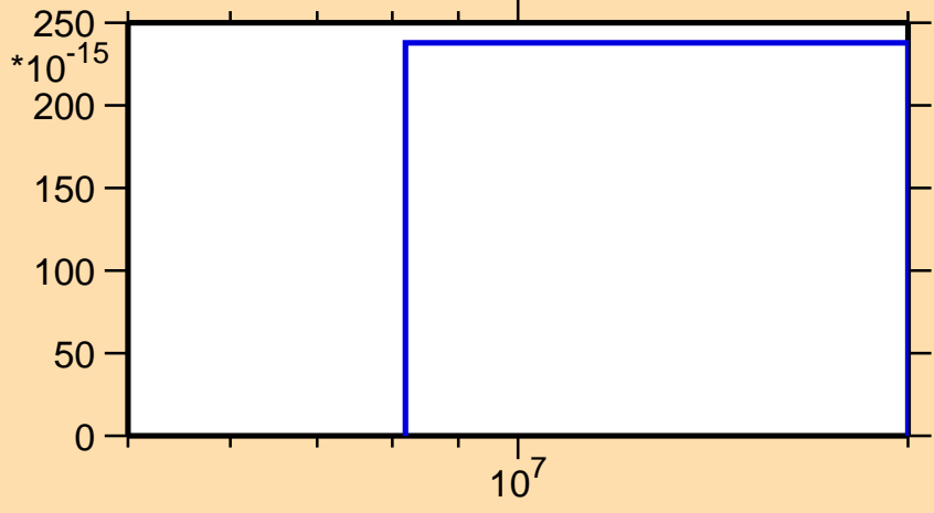
\sigma vs. E for ^{186}\text{Re}(n,p\alpha)
