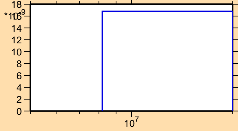
\sigma vs. E for ^{186}\text{Re}(n,nt)
