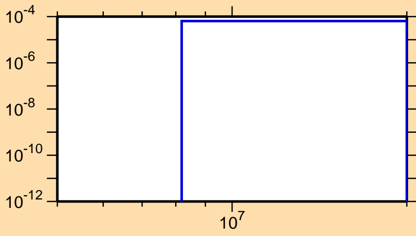
\sigma vs. E for ^{186}\text{Re}(n,t)
