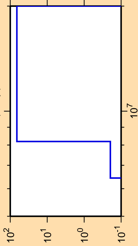
\Delta\sigma/\sigma vs. E for ^{186}\text{Re}(n,np)
