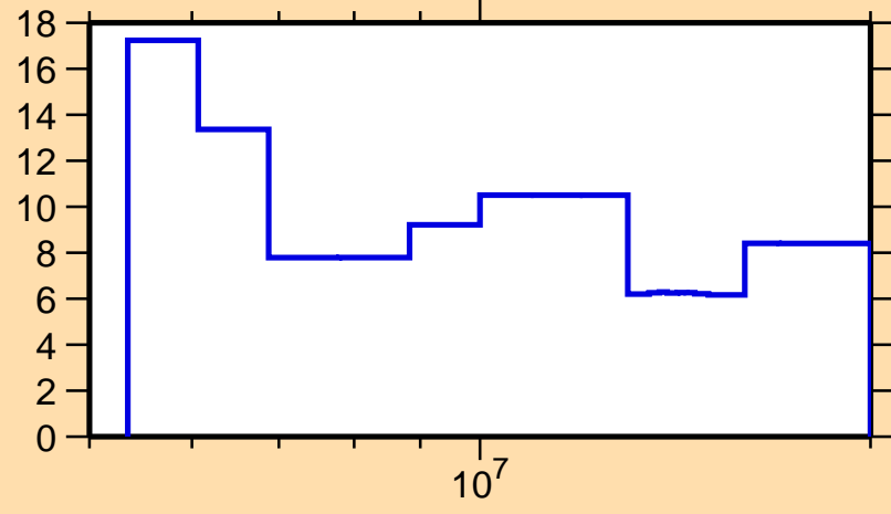
\Delta\sigma/\sigma vs. E for ^{186}\text{Re}(n,\text{el.})
