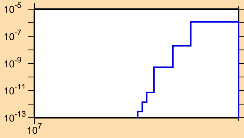
\sigma vs. E for ^{186}\text{Re}(n,nt)
