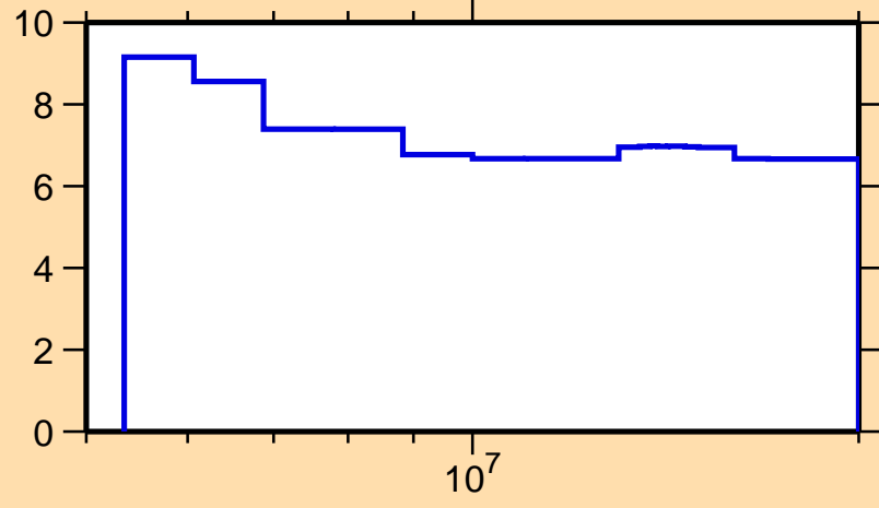
\Delta\sigma/\sigma vs. E for ^{186}\text{Re}(n,\text{nonel.})
