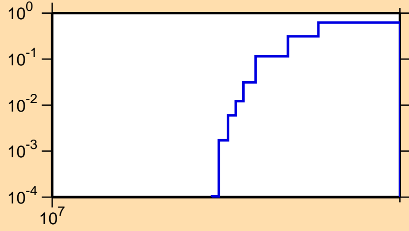
\sigma vs. E for ^{186}\text{Re}(n,3n)
