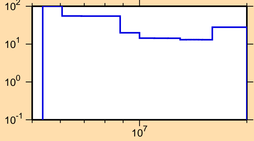
\Delta\sigma/\sigma vs. E for ^{186}\text{Re}(n,2n)
