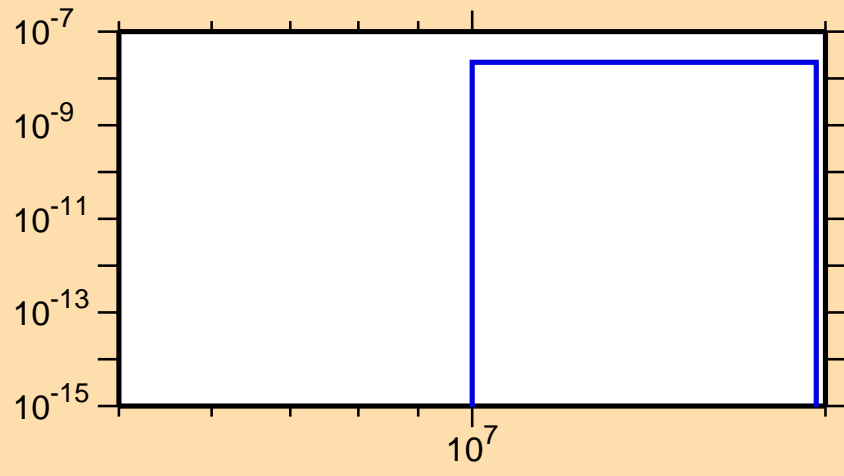
\sigma vs. E for ^{186}\text{Re}(n,2n\alpha)
