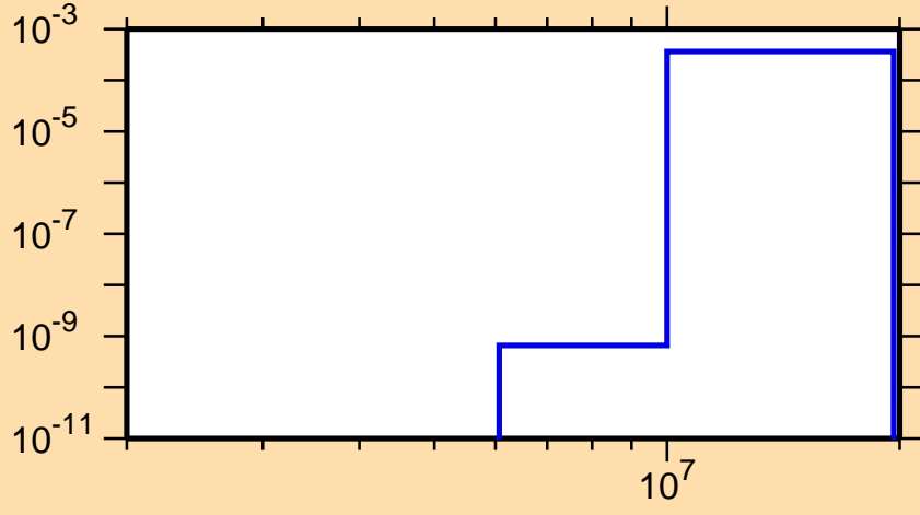
\sigma vs. E for ^{186}\text{Re}(n,np)
