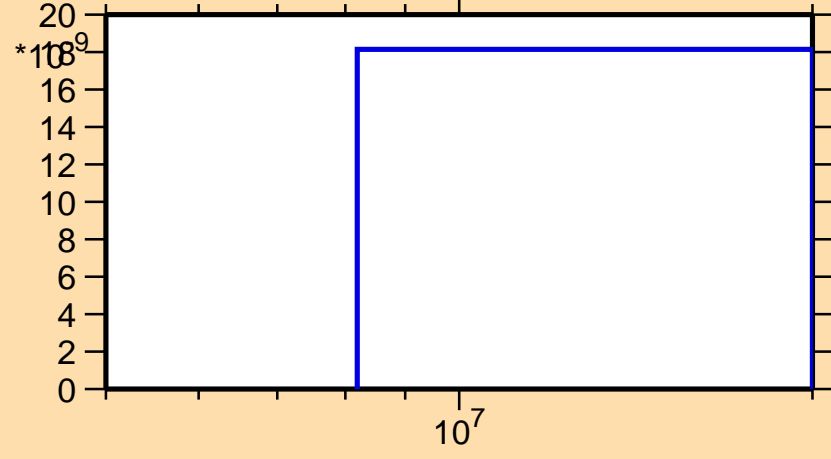
\sigma vs. E for ^{186}\text{Re}(n,2n\alpha)
