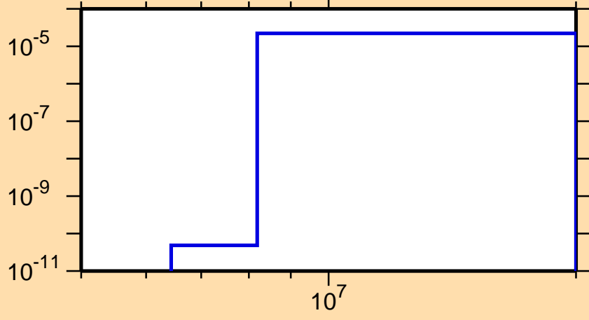
\sigma vs. E for ^{188}\text{Re}(n,\alpha)
