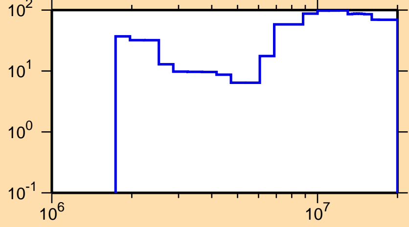
\Delta\sigma/\sigma vs. E for ^{188}\text{Re}(n,ncont.)
