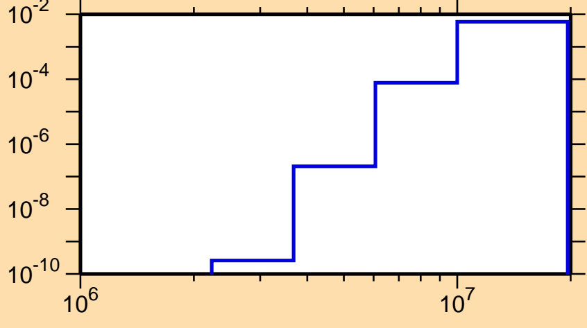
\sigma vs. E for ^{188}\text{Re}(n,p)
