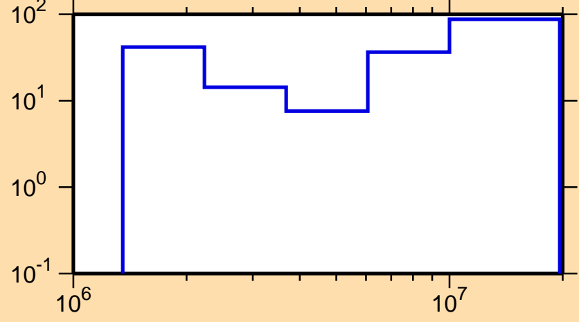
\Delta\sigma/\sigma vs. E for ^{188}\text{Re}(n,n\text{cont.})
