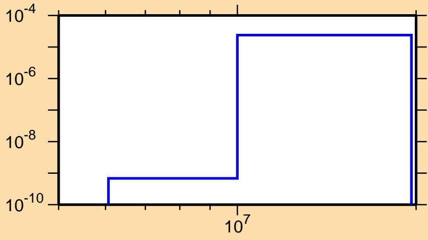
\sigma vs. E for ^{188}\text{Re}(n,\alpha)
