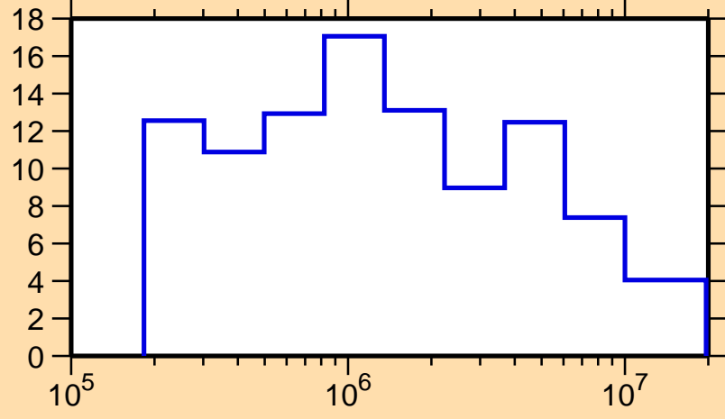
\Delta\sigma/\sigma vs. E for ^{188}\text{Re}(n, el.)
