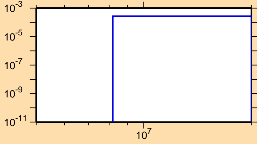
\sigma vs. E for ^{188}\text{Re}(n,d)
