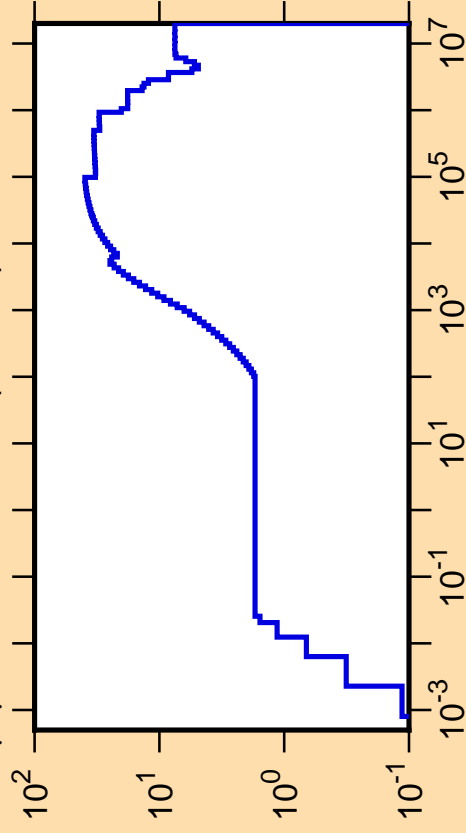
\Delta\mu/\mu vs. E for ^{189}\text{Re}(\text{mt251})
