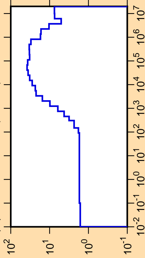
\Delta\mu/\mu vs. E for ^{189}\text{Re}(\text{mt251})
