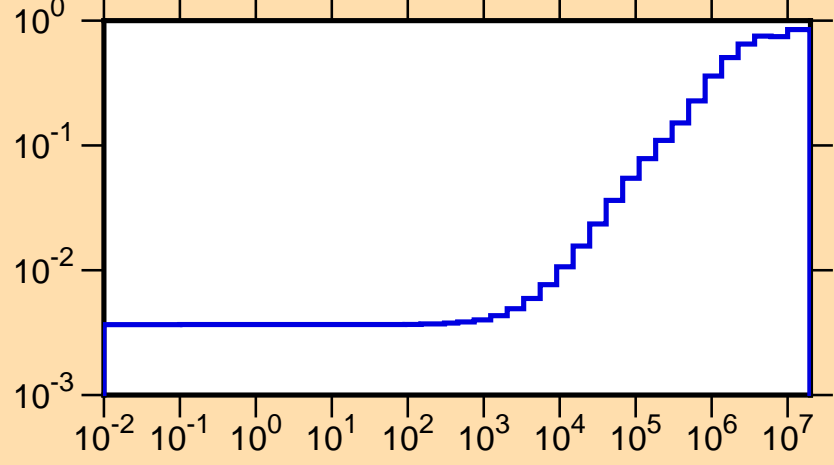
\mu vs. E for ^{189}\text{Re}(\text{mt251})
