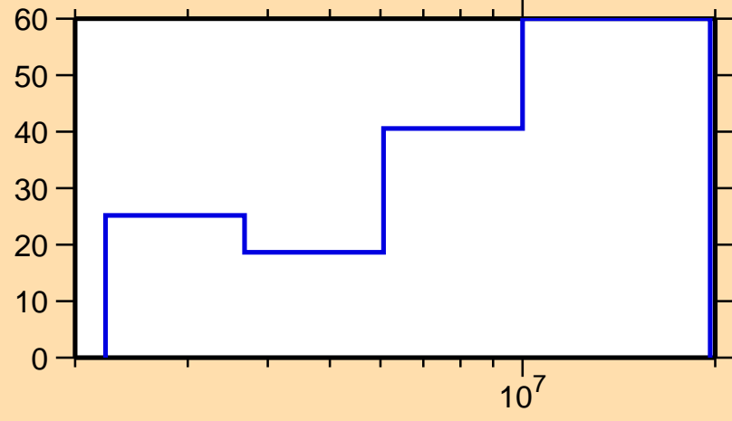
\Delta\sigma/\sigma vs. E for ^{189}\text{Re}(n,n\text{cont.})
