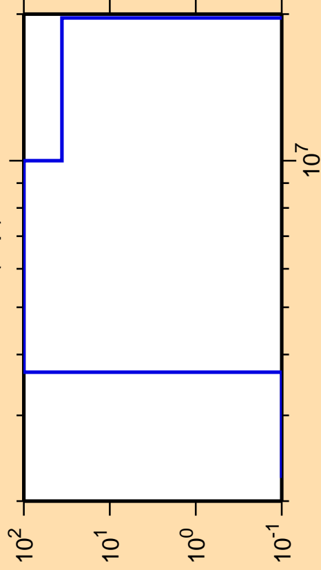
\Delta\sigma/\sigma vs. E for ^{189}\text{Re}(n,p)
