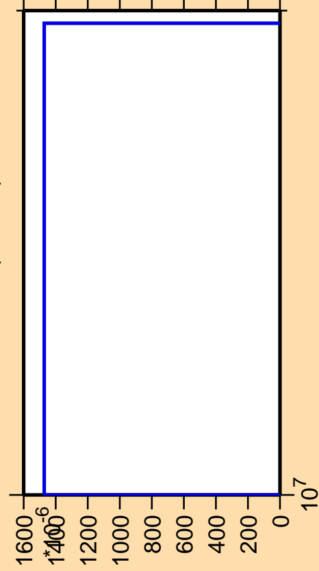
\Delta\sigma/\sigma vs. E for ^{189}\text{Re}(n,3n\alpha)
