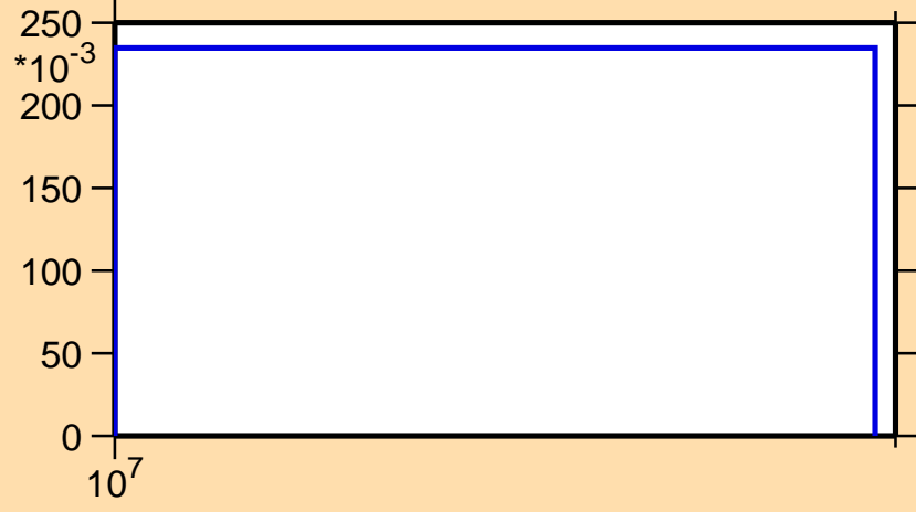
\sigma vs. E for ^{189}\text{Re}(n,3n)
