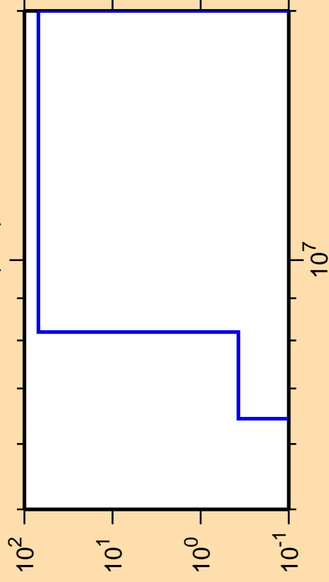
\Delta\sigma/\sigma vs. E for ^{189}\text{Re}(n,d)
