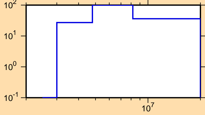
\Delta\sigma/\sigma vs. E for ^{189}\text{Re}(n,p)
