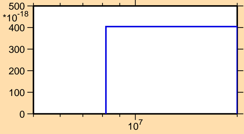
\sigma vs. E for ^{189}\text{Re}(n,3n\alpha)
