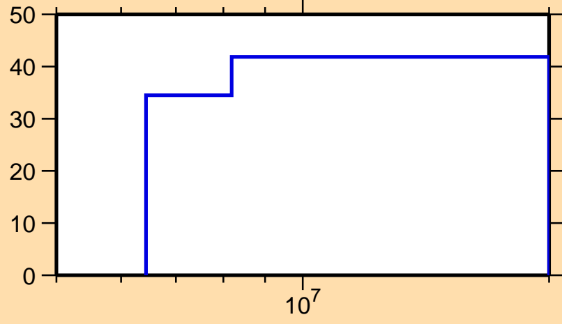
\Delta\sigma/\sigma vs. E for ^{189}\text{Re}(n,\text{inel.})
