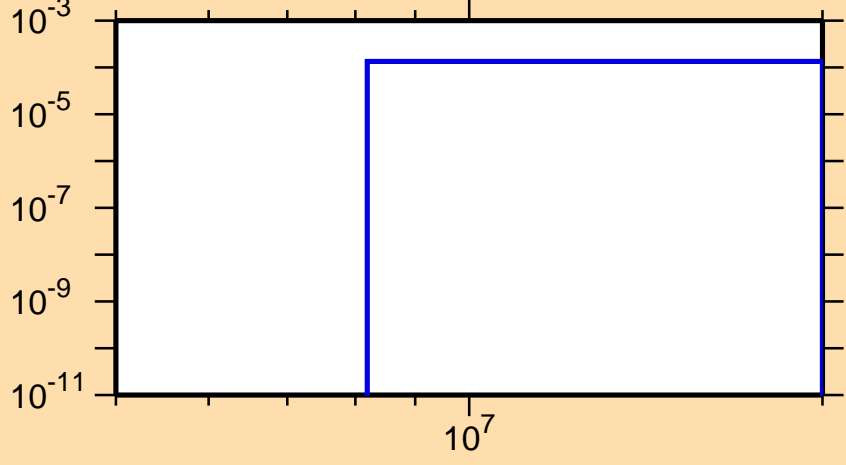
\sigma vs. E for ^{189}\text{Re}(n,d)
