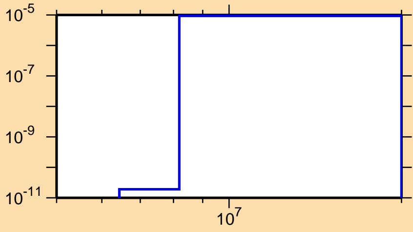
\sigma vs. E for ^{189}\text{Re}(n,\alpha)
