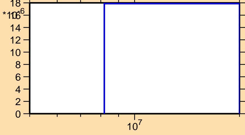
\sigma vs. E for ^{189}\text{Re}(n,t)
