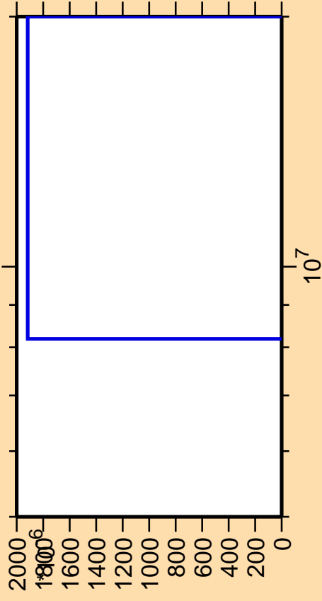
\Delta\sigma/\sigma vs. E for ^{189}\text{Re}(n,3n\alpha)
