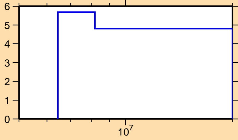
\Delta\sigma/\sigma vs. E for ^{189}\text{Re}(n,\text{el.})
