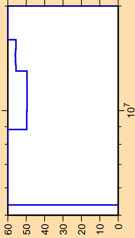
\Delta\sigma/\sigma vs. E for ^{190}\text{Re}(n,\gamma)
