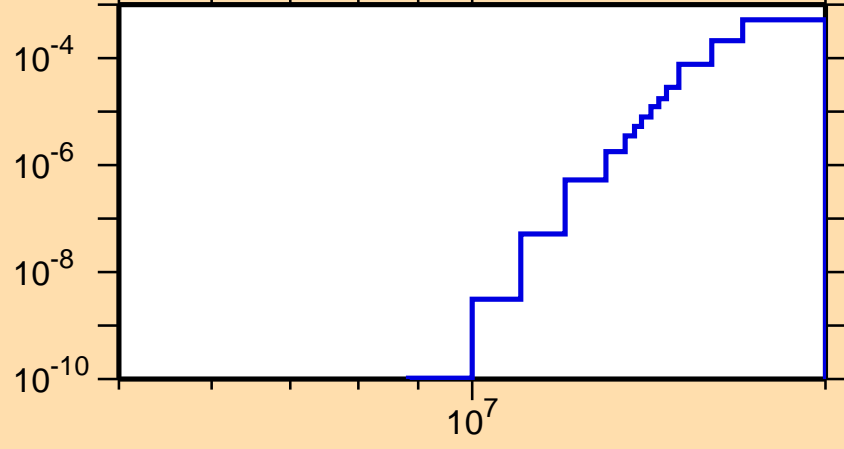
\sigma vs. E for ^{190}\text{Re}(n,t)
