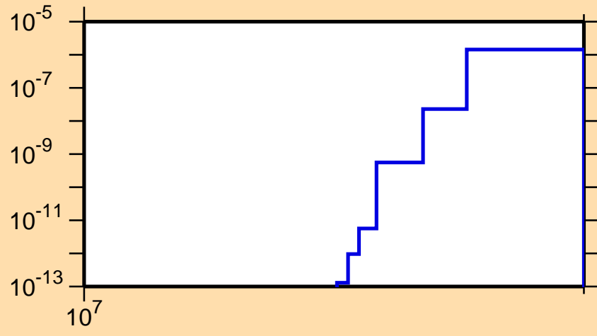
\sigma vs. E for ^{190}\text{Re}(n,nt)
