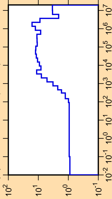
\Delta\mu/\mu vs. E for ^{190}\text{Re}(\text{mt251})
