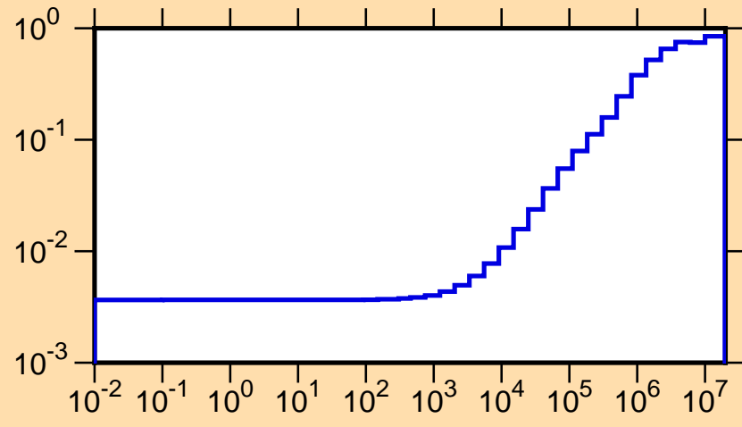
\mu vs. E for ^{190}\text{Re}(\text{mt251})
