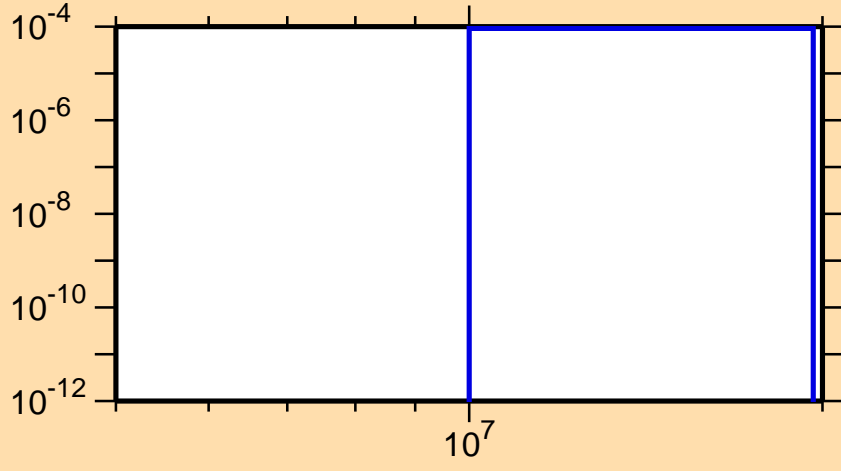
\sigma vs. E for ^{190}\text{Re}(n,np)
