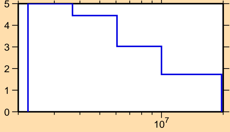
\Delta\sigma/\sigma vs. E for ^{190}\text{Re}(n,\text{nonel.})
