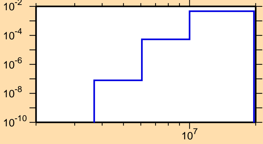
\sigma vs. E for ^{190}\text{Re}(n,p)
