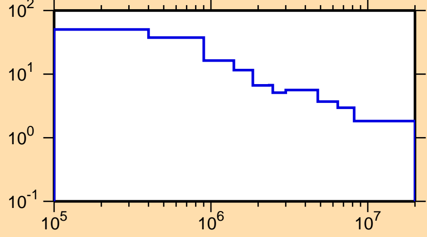
\Delta\sigma/\sigma vs. E for ^{190}\text{Re}(n,\text{nonel.})
