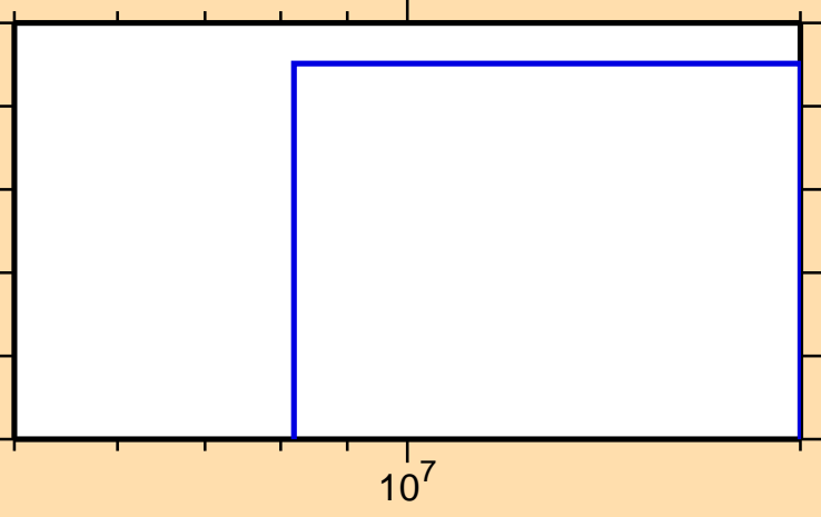
\sigma vs. E for ^{190}\text{Re}(n,3n)
