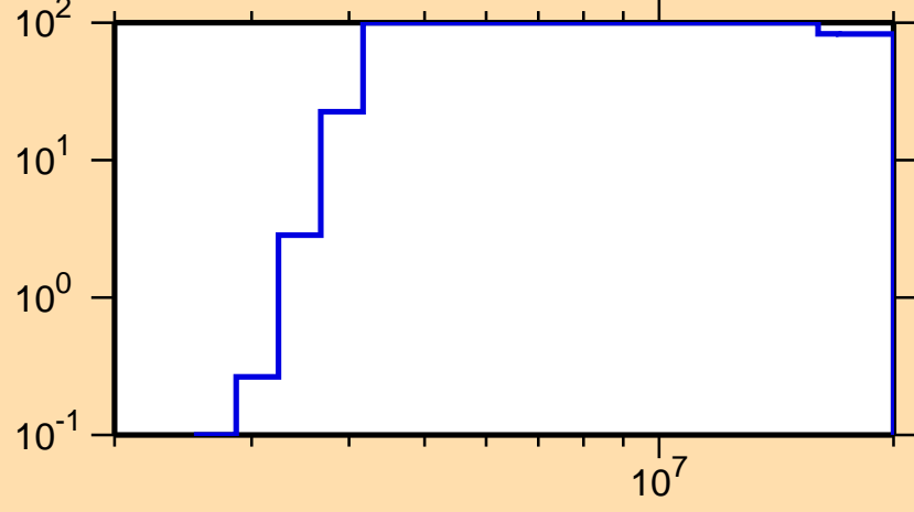
\Delta\sigma/\sigma vs. E for ^{190}\text{Re}(n,p)
