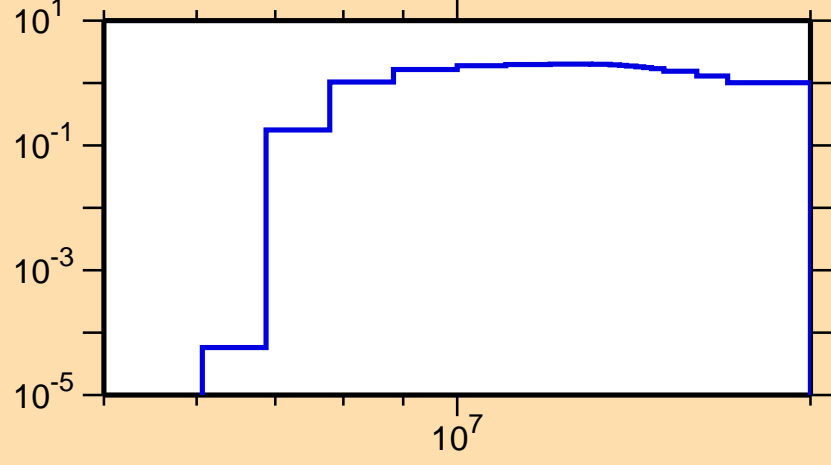
\sigma vs. E for ^{191}\text{Re}(n,2n)
