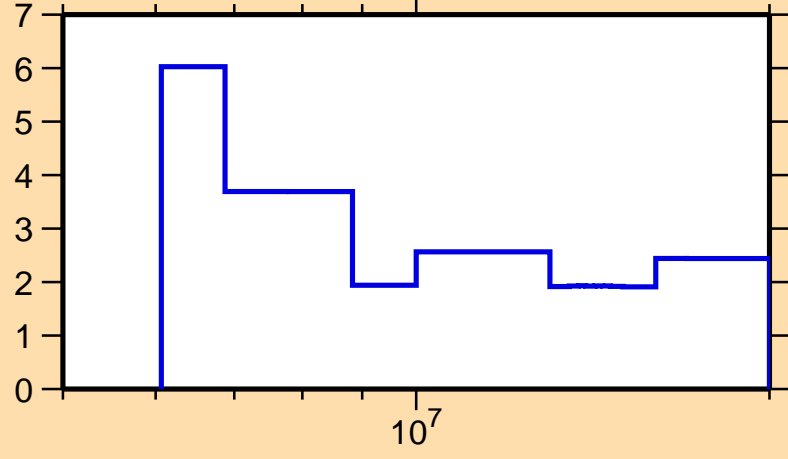
\Delta\sigma/\sigma vs. E for ^{191}\text{Re}(n,\text{tot.})
