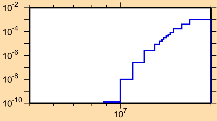
\sigma vs. E for ^{191}\text{Re}(n,d)
