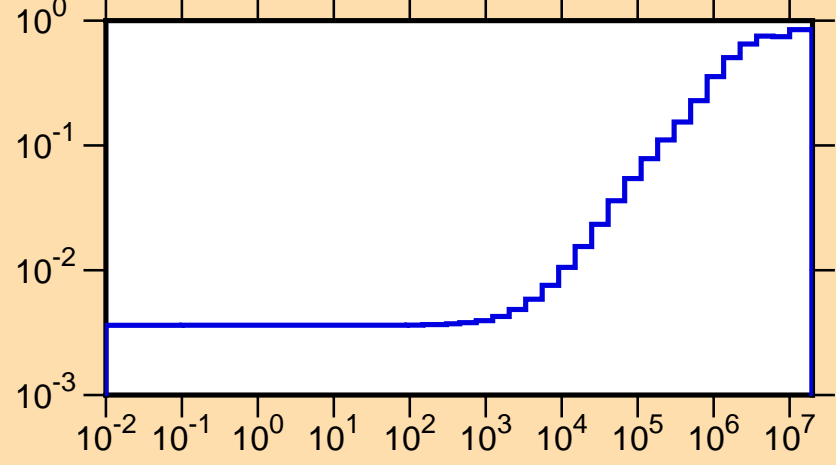
\mu vs. E for ^{191}\text{Re}(\text{mt251})
