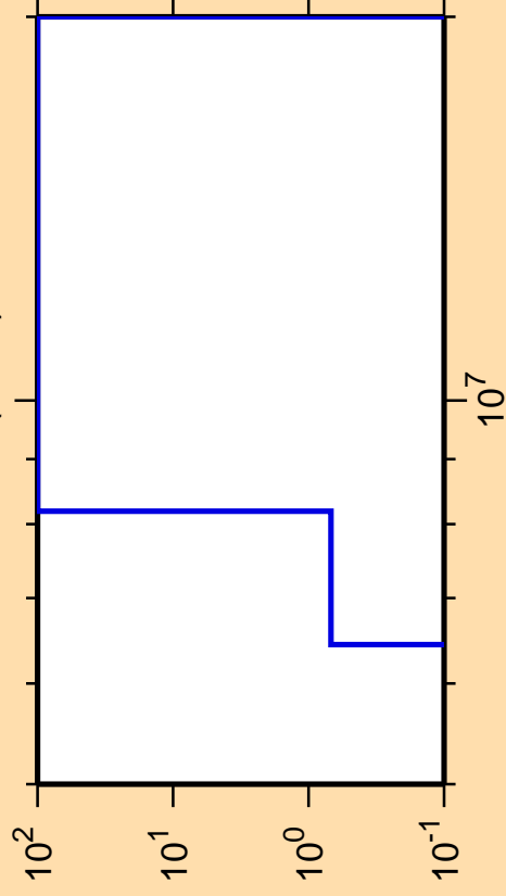
\Delta\sigma/\sigma vs. E for ^{191}\text{Re}(n,\alpha)
