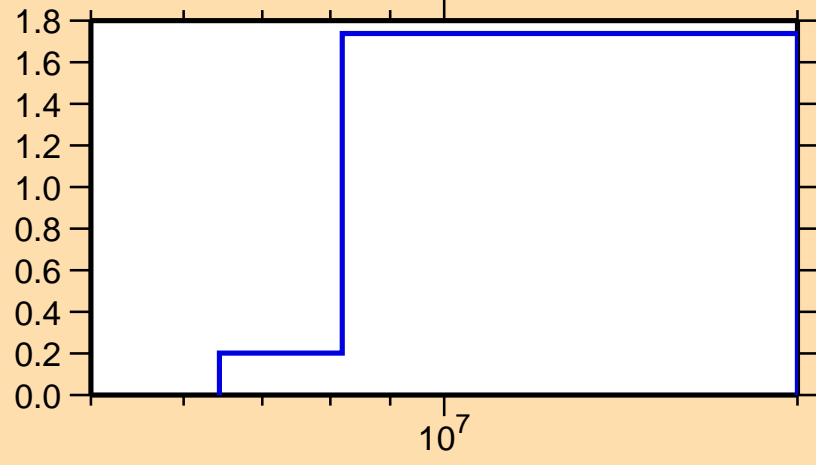
\sigma vs. E for ^{191}\text{Re}(n,2n)
