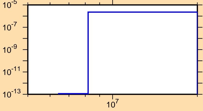
\sigma vs. E for ^{191}\text{Re}(n,\alpha)
