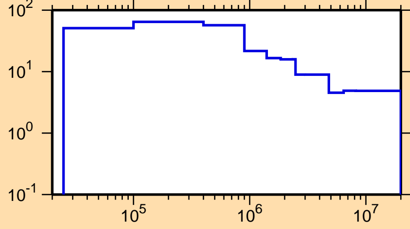
\Delta\sigma/\sigma vs. E for ^{191}\text{Re}(n,\text{nonel.})
