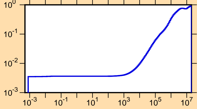
\mu vs. E for ^{192}\text{Re}(\text{mt251})
