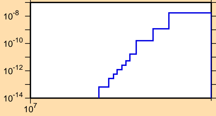
\sigma vs. E for ^{192}\text{Re}(n,2n\alpha)
