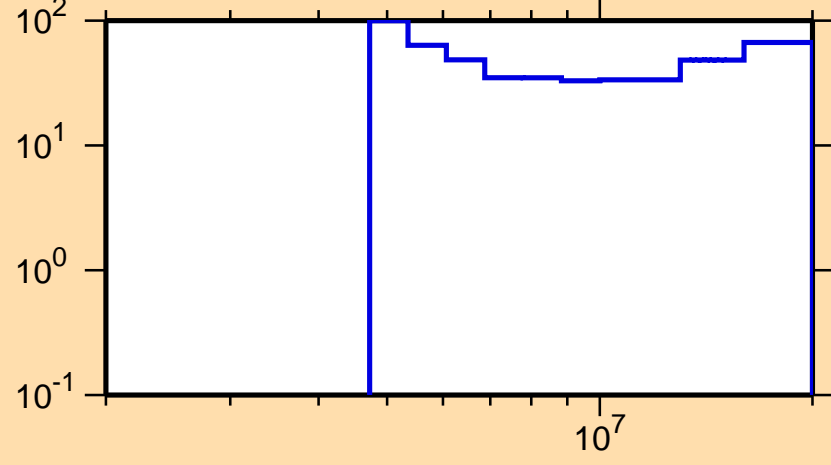
\Delta\sigma/\sigma vs. E for ^{192}\text{Re}(n,2n)
