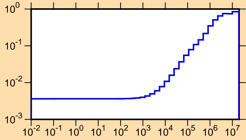
\mu vs. E for ^{192}\text{Re}(\text{mt251})
