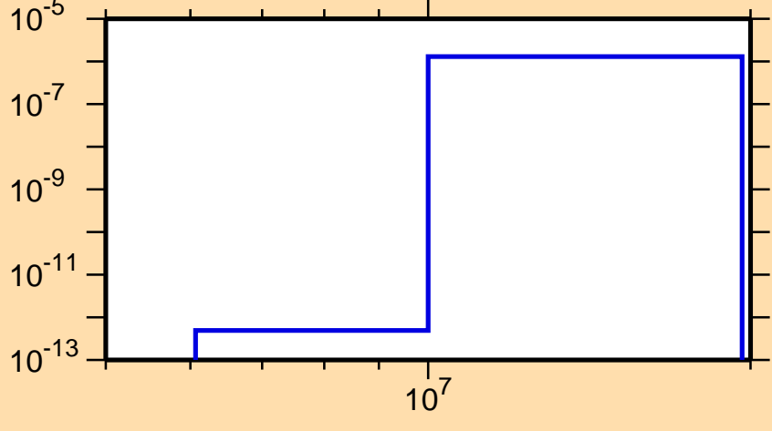
\sigma vs. E for ^{192}\text{Re}(n,\alpha)
