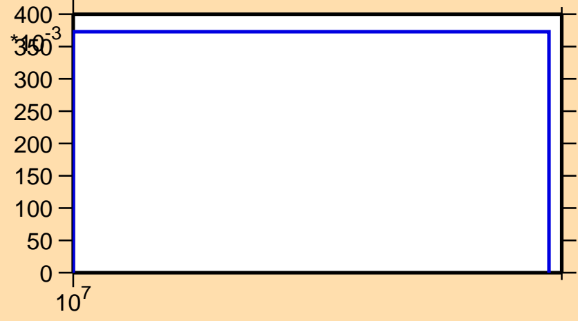
\sigma vs. E for ^{192}\text{Re}(n,3n)
