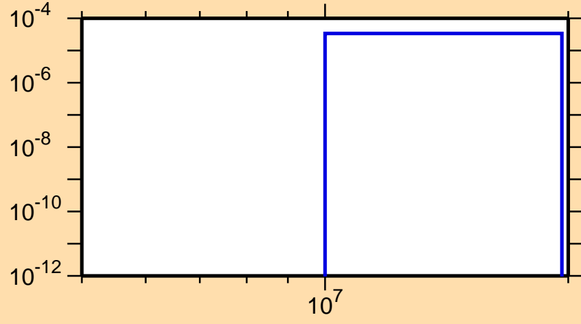
\sigma vs. E for ^{192}\text{Re}(n,np)
