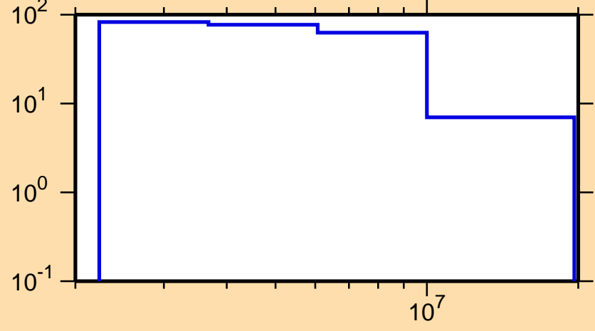
\Delta\sigma/\sigma vs. E for ^{192}\text{Re}(n,n_1)
