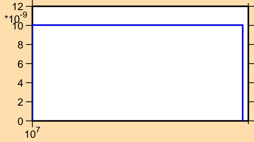
\sigma vs. E for ^{192}\text{Re}(n,\text{nd})
