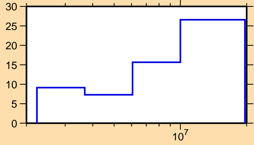
\Delta\sigma/\sigma vs. E for ^{192}\text{Re}(n,el.)
